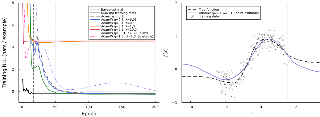
Figure 10: Left : Training NLL vs. epoch for DMA (solid black), Adam \eta = 0.1 (dashed grey), AdamW \eta = 0.1 at four weight decay values (solid coloured), and two poorly-tuned AdamW configurations ( \eta = 0.01 and \eta = 1.0 , both \lambda = 1.0 , dotted) illustrating hyperparameter sensitivity. Right : AdamW \eta = 0.1 , \lambda = 0.1 (best weight decay on this seed) point prediction outside the training range [-2.5, 1.5] (dotted verticals); the true function (dashed) is tracked well on this seed but no uncertainty quantification is available.
