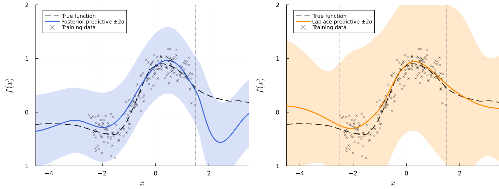
Figure 14: Left : DMA posterior predictive (same as Figure 2). Right : Diagonal Laplace predictive with He-init prior (MAP via Adam with per-layer L_2 decay, diagonal of exact Hessian, K = 1000 MC samples). Training range [-2.5, 1.5] marked by dotted verticals.
