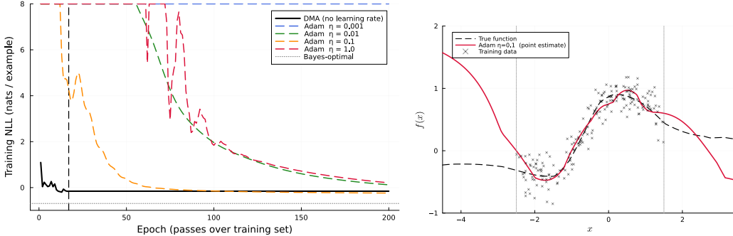
Figure 9: Left: Training negative log-likelihood ( \text{NLL} = -\frac{1}{N} \sum_i \log p(y_i | x_i) , nats/example) versus epoch for DMA (solid black) and Adam at four learning rates (dashed). DMA’s outer updates stop automatically at epoch 17; Adam’s speed and final NLL depend critically on \eta . Values above 8 are clipped to 8 for display. Right: Adam ( \eta = 0.1 ) point prediction outside the training range [-2.5, 1.5] (dotted verticals); the true function (dashed) can deviate arbitrarily from the point estimate, with no uncertainty quantification available. Compare with the widening DMA posterior in Figure 2. DMA’s per-epoch cost is 0.80 ms versus 0.45 ms for Adam on this architecture ( 1.8\times ), but DMA’s early stopping at epoch 17 versus Adam’s \sim 80 gives an overall \sim 5\times reduction in total training time.
