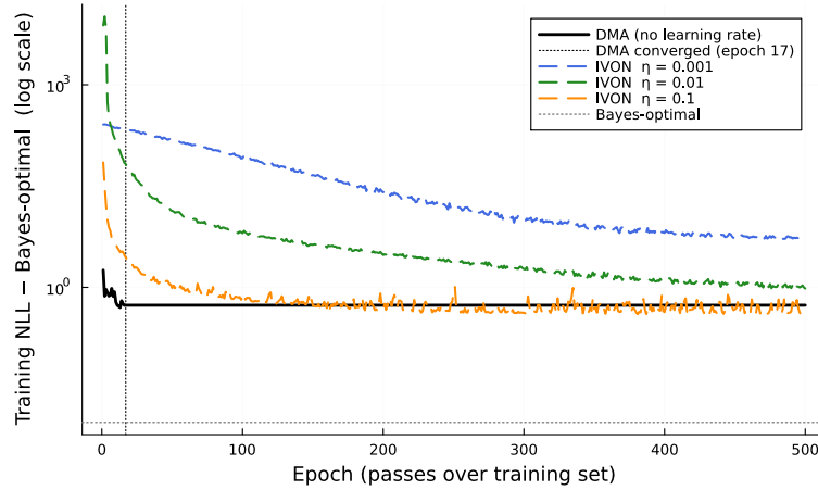
Figure 12: Training NLL minus Bayes-optimal (log scale) vs. epoch for IVON at three learning rates (best \beta_2/\delta per \eta from the sweep) and DMA, on the 83-weight BNN ( N=200 , \beta=0.2 ). DMA converges at epoch 17; \eta=0.001 descends slowly but does not converge within 500 epochs; \eta=0.01 converges to \text{NLL} \approx 0.26 with \delta=0.5 ; \eta=0.1 oscillates near the Bayes-optimal line.
