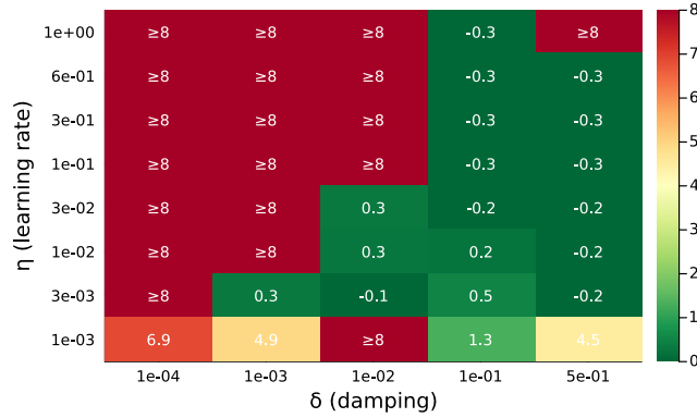
Figure 11: Hyperparameter sweep: minimum training NLL achieved over 500 epochs for each of 160 IVON configurations ( 8 \times 4 \times 5 grid over \eta , \beta_2 , \delta ) on the 83-weight BNN ( N=200 , \beta=0.2 ). Only 26 of 160 configurations reach a final NLL below 1.0, concentrated in the \delta=0.1 and \delta=0.5 columns. DMA training NLL at convergence: -0.16 (epoch 17, no hyperparameter search); best IVON: -0.31 (epoch 500, requires \delta=0.1 and extensive tuning).
