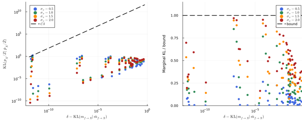
Figure 3: Empirical validation of Theorem 2.3 across 192 leaky-ReLU factor configurations. Left : log-log scatter of message error \delta versus marginal error; the dashed line C\delta (with C = \|m_{X_j \rightarrow f}\|_\infty / Z ) lies above every point, confirming O(\delta) scaling. Right : the marginal KL normalised by its per-configuration bound \|m_{X_j \rightarrow f}\|_\infty / Z \cdot \delta ; all 192 ratios lie below the bound line at 1 (maximum ratio 0.97), directly certifying the theorem. The bound is tight: the \|m_{X_j \rightarrow f}\|_\infty / Z prefactor evaluates the Gaussian sup-norm, which is largest where the incoming message is most concentrated and the marginal error is therefore small anyway.
