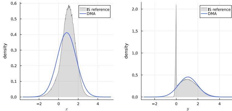
Figure 8: ReLU / Leaky-ReLU factor ( \alpha = 0.1 ), nominal scenario ( \mu_X = 1, \sigma_X^2 = 1 ). Left: backward marginal X . Right: forward marginal Y . Blue: DMA, Gray: IS reference
