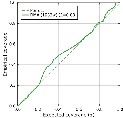
Figure 21: Extrapolation calibration curve for DMA on the 1932-weight network ( N = 1500 ), averaged across all four output channels. Test points in [-6, -4] \cup [4, 6] . \Delta = +0.026 (slightly conservative); the 83-weight result has a 20-seed median \Delta = -0.09 (Appendix E.7).
