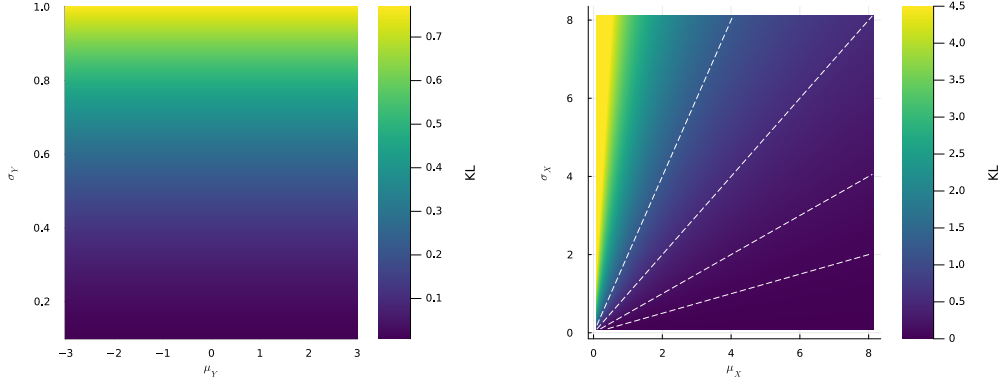
Figure 6: Copy-factor KL divergence over the 2D parameter space, computed from the closed-form expression in Lemma B.3 (no Monte Carlo). Left : Step 1 error KL[\text{LN}(\cdot; \mu_Y, \sigma_Y^2), \hat{m}_{f \rightarrow X}(\cdot)] swept over (\mu_Y, \sigma_Y) . Horizontal bands confirm that the KL depends only on the log-space variance \sigma_Y^2 , not on \mu_Y ; the analytical rate is \frac{3}{4}\sigma_Y^2 + O(\sigma_Y^4) . Right : Step 2 error KL[\text{LN}_m(\cdot; \mu_X, \sigma_X^2), \mathcal{N}(\cdot; \mu_X, \sigma_X^2)] swept over (\mu_X, \sigma_X) . Dashed white lines are level curves of r = \mu_X/\sigma_X ; diagonal banding confirms the KL depends only on r , consistent with the O(1/r^2) rate.
