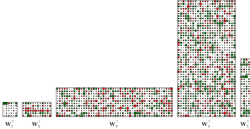
Figure 19: Hinton diagram of DMA posterior weight means after 3 epochs. Each block corresponds to one weight matrix; square size encodes |\mu_w| , colour encodes sign.
