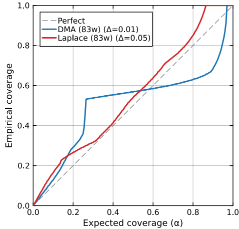
Figure 15: Extrapolation calibration curves for the 83-weight network, test points in [-4, -2.5] \cup [1.5, 3] . \Delta = \text{coverage} - \alpha : 0 = perfect, > 0 = conservative, < 0 = overconfident. On this seed, DMA (blue, \Delta = +0.01 ) and diagonal Laplace (red, \Delta = +0.05 ); \Delta is the mean signed deviation — DMA’s smaller |\Delta| reflects cancellation of over- and under-coverage rather than a uniformly tighter fit to the diagonal. Over 20 seeds both methods are comparable (median -0.09 vs. -0.10 ).
