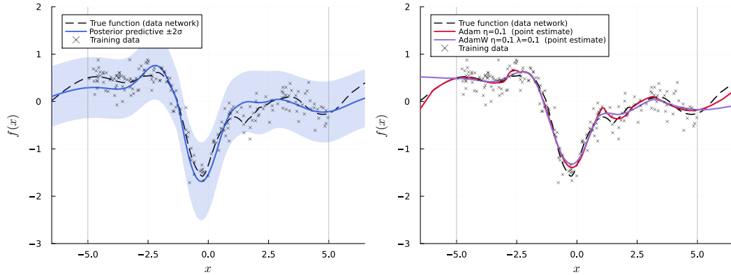
Figure 16: Model mismatch experiment ( N = 200 , training range [-5, 5] , \beta = 0.2 ). The data-generating network has two wider hidden layers ( d = 12, 10 ); both methods learn with the two-hidden-layer model network ( d = 6, 5 ). Left : DMA posterior predictive mean (solid) and \pm 2\sigma intervals (shaded) versus the true function (dashed). Training points are shown as crosses; dotted vertical lines mark the training boundaries x = \pm 5 . Right : Adam ( \eta = 0.1 , red) and AdamW ( \eta = 0.1, \lambda = 0.1 , purple) point predictions; neither carries uncertainty quantification.
