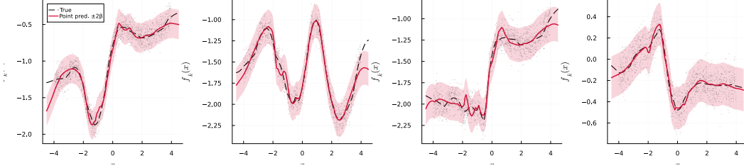
Figure 18: Adam ( \eta = 0.01 , 100 epochs, 1.7 s total) point predictions with fixed \pm 2\beta bands on the same four output channels. The confidence interval is constant across the input range because a point estimate carries no epistemic uncertainty.
