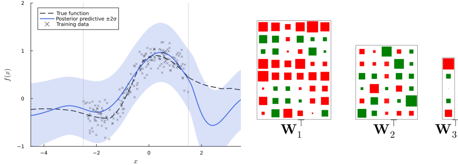
Figure 2: Left : Posterior predictive mean (solid) and \pm 2\sigma intervals (shaded) versus the true data-generating function (dashed), where \sigma = \sqrt{\text{Var}[f(x)] + \beta^2} combines posterior variance with observation noise ( \beta=0.2 ). Training points shown as crosses ( N = 200 , x \in [-2.5, 1.5] ); dashed verticals mark the training boundaries. Right : Hinton diagram of posterior weight beliefs after training. Square area \propto posterior mean magnitude; transparency \propto posterior variance (opaque = certain).
