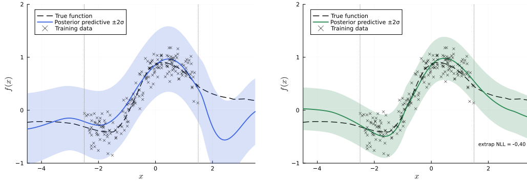
Figure 13: Left : DMA posterior predictive (identical to Figure 2). Right : IVON predictive with the best sweep configuration ( \eta=0.6 , \beta_2=0.9999 , \delta=0.1 ) after 2000 epochs. Training range [-2.5, 1.5] marked by dotted verticals. DMA extrapolation NLL: 0.54; IVON on this seed: -0.40 . Across 20 seeds IVON diverges on 14/20; median extrap NLL on finite seeds is 2.11 (IQR 5.27) vs. DMA median 0.79 (IQR 1.28).
