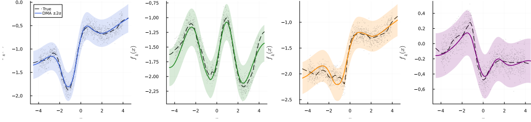
Figure 17: DMA posterior predictive (6→6→12→48→24→4, 1932 weights, N = 1500 , 3 epochs, 0.72 s total). Each panel shows one of the four output channels: posterior predictive mean (solid) with \pm 2\sigma bands against the true function (dashed); training points as faint dots.
