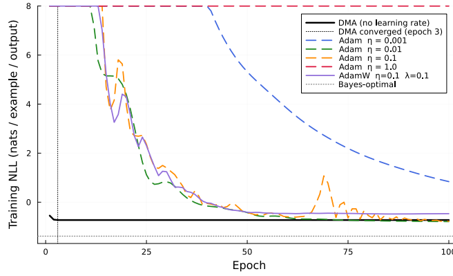
Figure 20: Training NLL (per example per output) vs. epoch. DMA (solid black) converges at epoch 3 with no learning-rate tuning. Adam with \eta = 0.01 reaches NLL -0.79 after 100 epochs; \eta = 0.001 has not converged (NLL +0.84 ); \eta = 1.0 diverges. Values above 8 are clipped to 8 for display. AdamW \eta = 0.1 , \lambda = 0.1 (solid purple) reaches NLL -0.47 : weight decay regularises the trajectory but the chosen \eta does not reach the same final NLL as the best-tuned Adam.
