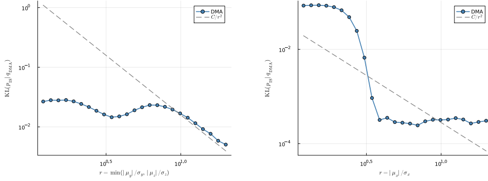
Figure 5: KL divergence between IS reference marginal and DMA marginal as a function of input SNR r . Left : product factor backward message to X from Z = XY ; incoming messages Y \sim \mathcal{N}(\mu_y, (\mu_y/r)^2) and Z \sim \mathcal{N}(\mu_z, (\mu_z/r)^2) with \mu_y = 4 , \mu_z = 10 , and the incoming message from X fixed at \mathcal{N}(3, 1) . Right : ReLU backward message to X from Y = \text{relu}(X; \alpha) with \alpha = 0.1 ; incoming message X \sim \mathcal{N}(\mu_x, (\mu_x/r)^2) with \mu_x = 1 . Both panels show empirical O(1/r^2) decay. The product backward (left) is covered by Theorem 3.3; the leaky-ReLU backward (right, \alpha=0.1 , proper message) is consistent with Theorem 2.3 applied to the message KL.
