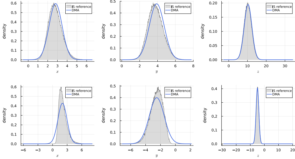
Figure 7: Product factor f(X, Y, Z) = \delta(Z - XY) . Each row shows marginals X, Y, Z (left to right). Blue: DMA. Gray: IS. (a) Nominal ( \mu_X = 3, \sigma_X^2 = 1, \mu_Y = 4, \sigma_Y^2 = 1, \mu_Z = 10, \sigma_Z^2 = 5 ): the Z forward marginal is well approximated by the DMA Gaussian; the X and Y backward marginals are already noticeably skewed in the IS reference. (b) Stress ( \mu_X = 1, \sigma_X^2 = 4, \mu_Y = -2.5, \sigma_Y^2 = 1, \mu_Z = -5, \sigma_Z^2 = 1 ): Z remains well approximated; the X and Y backward marginals become severely non-Gaussian.
