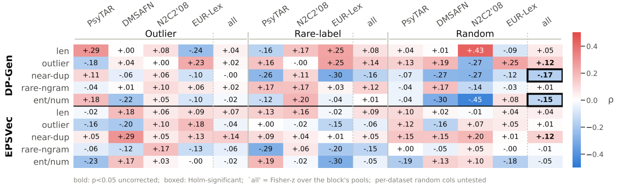
Figure 5: Full attribute-vulnerability matrix: the outlier and rare-label pools alongside the random pools of Figure 4. Cell format and significance marks as there; within each block, all is the Fisher-z pool with Holm correction over the block’s five attributes. None of the 70 per-pool tests in the selected pools reaches nominal significance. Outlierness is range-restricted in the outlier pools, which are selected on that statistic.
