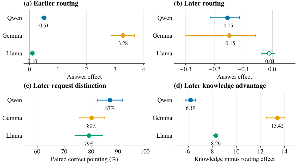
Figure 6: Deletion of the fitted global request direction causes less answer damage in fixed later layer sets, while fitted-content deletion remains consequential. All three models use the same 24 new country pairs but model-specific layer sets fixed before this evaluation: Qwen {29, 31} versus {32, 34}, Gemma {24} versus {25, 30}, and Llama {15, 24} versus {28}. Request states remain separable along the late global direction. Bars show 95% country-pair bootstrap intervals; a hollow marker denotes an interval spanning zero. The figure concerns this global fitted direction, not all request representations or a shared processing boundary.
