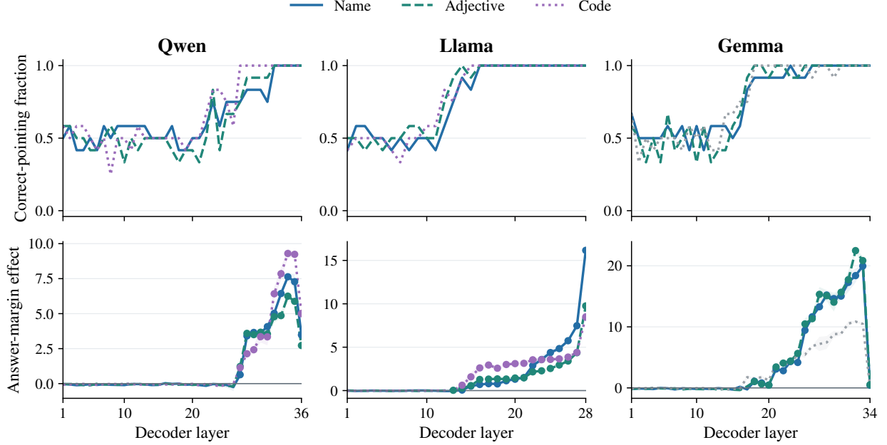
Figure 4: Answers become sensitive to deleting fitted continent content, and that sensitivity persists in late layers. Top: the fraction of questions whose projected state is closer to the requested continent reference than to the paired alternative. Bottom: mean answer-margin damage from deleting that projection, corrected by matched random changes. Each model, layer, and answer format has its own fitted two-dimensional space. Lines and shading show the mean and range of validation A and B, not confidence intervals; filled dots require positive effects in screening and both validation splits. Gemma code results are diagnostic and shown in gray. In the original final-layer point, reading occurs after final normalization but intervention occurs before it; Appendix C provides location-aligned block-output profiles, and the original final drop is not interpreted as content disappearance.
