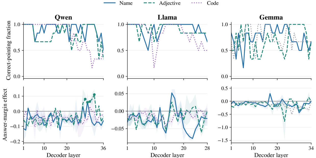
Figure 3: Transferred selection has a task-dependent layerwise effect. Top: the paired-request correct-pointing fraction of the transferred selection direction. Bottom: its deletion effect on the answer margin relative to eight matched random changes. Lines average the two validation partitions; shading spans their values. Filled dots identify layers passing both auxiliary calibration and positive-effect checks in all three evaluated partitions. Other values are retained, including negative values. Gray dotted Gemma code curves are diagnostic because baseline qualification failed. These are effects after transfer to continent questions, not the marker-calibration switching rates.
