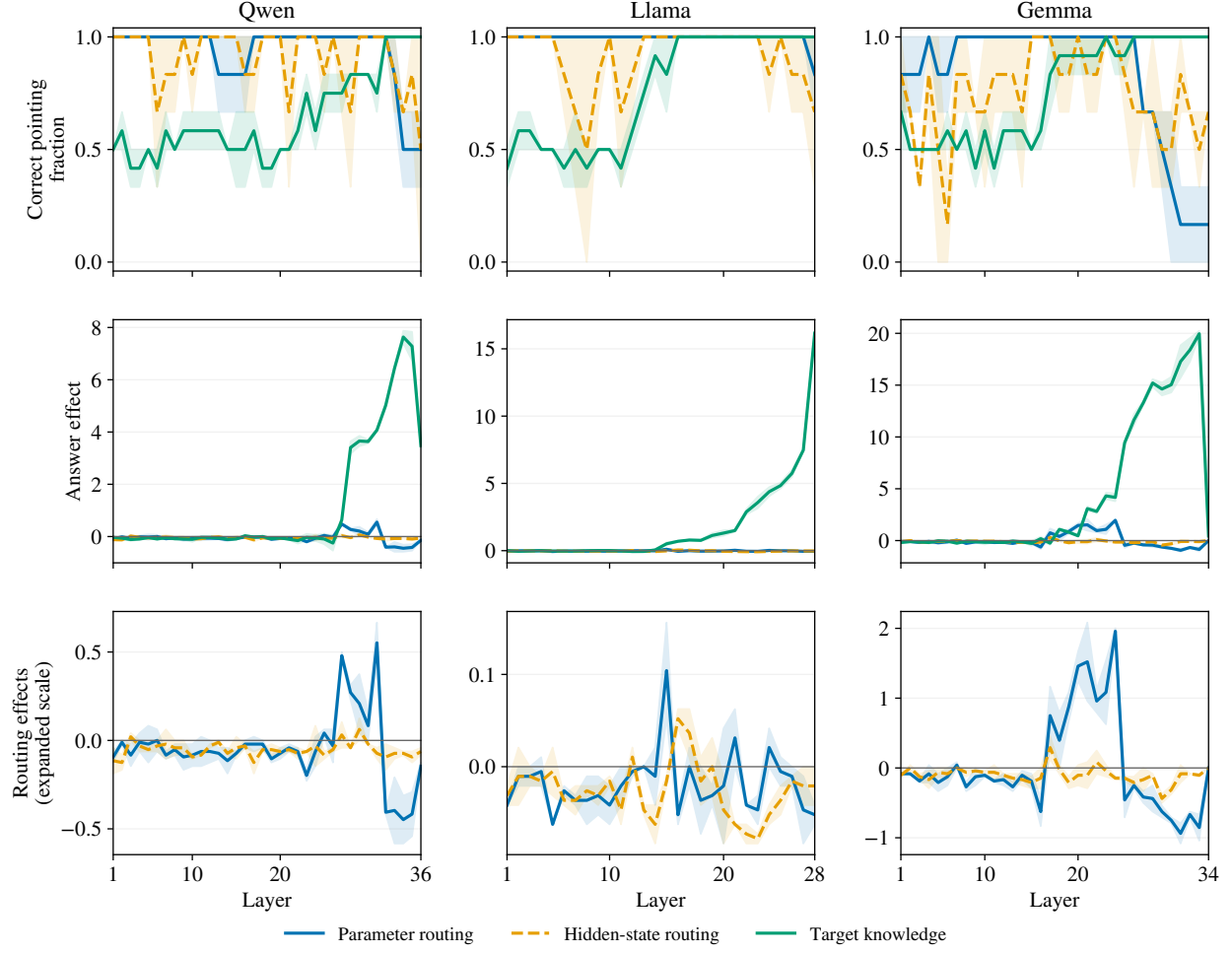
Figure 8: Three-component profiles on continent-name questions. Top: correct-pointing fractions. Middle: random-corrected deletion effects on the answer. Bottom: the same routing effects with an expanded vertical scale, without normalization. Lines average validation A and B; shading spans their two values. Orange dashed selection curves include unqualified layers. The presence of a curve does not assert a stable effect.
