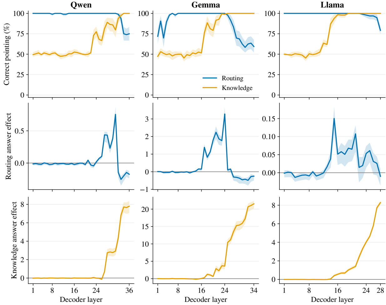
Figure 12: Expanded depth profiles on 24 new country pairs. Top: paired routing correct-pointing fractions and target-knowledge correct-pointing fractions. Middle: routing answer effects. Bottom: target-knowledge answer effects. Shading gives pointwise 95% country-pair bootstrap intervals; it differs from the two-partition ranges in Figure 8. Each column uses its model’s full decoder depth and separately fitted components. Routing and knowledge effects have separate vertical scales.
