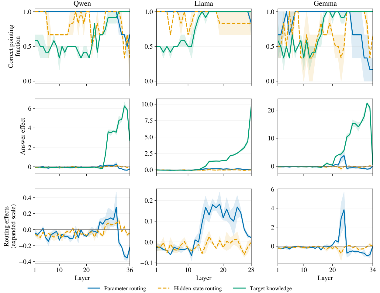
Figure 10: Adjective-format lifecycle. Layout and measurements follow Figure 8. Lines average the two validation results; shading is their range, not a confidence interval. The bottom row expands the routing scale without normalization. Dashed orange lines show the transferred selection candidate, including unqualified layers. Stable effects require the additional criteria in Section A; readable or positive values alone do not qualify a layer.
