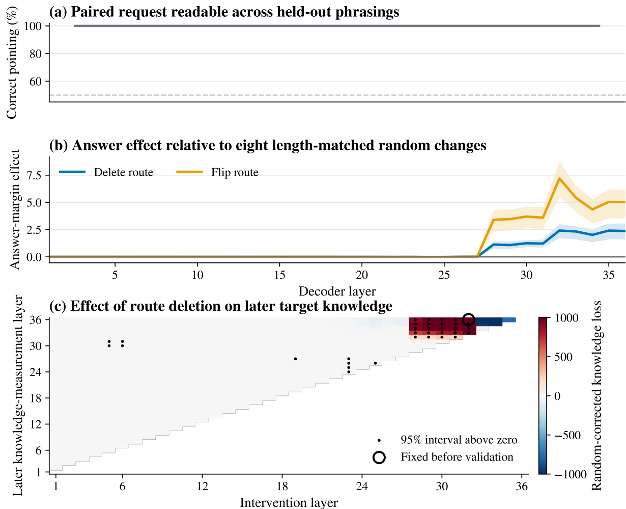
Figure 1: A readable pair-conditioned request distinction and detectable answer dependence have different depth profiles in Qwen. Every model input is a single-country question; two countries are paired only for analysis. Template A constructs one direction per pair, and two held-out phrasings evaluate it on 24 new pairs. (a) Correct pointing is the fraction of questions for which the coefficient sign identifies the queried pair member. (b) Answer effect is the mean correct-versus-paired margin loss minus the largest mean loss among eight random changes matched to the actual intervention length. Lines show estimates; bands show 95% country-pair bootstrap intervals. (c) Color shows the similarly corrected loss of the fitted continent score at a later layer after source-layer deletion. Black dots mark individual layer pairs whose 95% interval lies above zero, not a simultaneous matrix test. The circle marks source layer 32 and receiver layer 36, fixed before validation. Deletion at that pair has an interval spanning zero for later knowledge, whereas reversal passes. Values use float32 and are not compared in magnitude with the bfloat16 paired-task experiments.
