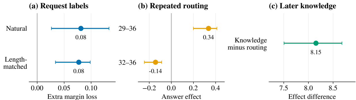
Figure 7: Qwen controls test request specificity and repeated deletion. (a) The true request direction exceeds the strongest of nine balanced wrong-label directions, averaged over layers 29 and 31. (b) Repeated routing-deletion effects use random paths matched to the actual lengths after numerical rounding. (c) Repeated late content deletion exceeds repeated late routing deletion. Points and 95% intervals use the same 24 country pairs. The single-versus-repeated comparison concerns the measured direction, not every possible representation of a request.
