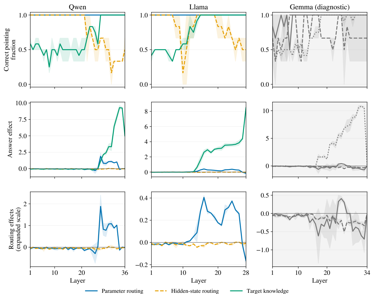
Figure 11: Code-format lifecycle. Layout and measurements follow Figure 8. Gemma’s gray column is diagnostic because this model–format combination failed behavioral qualification. Within that column, solid, dashed, and dotted lines denote parameter routing, hidden-state routing, and target knowledge, respectively. Shading is the range of the two validation results, not a confidence interval. Diagnostic values are retained rather than treated as confirming the main conclusions.
