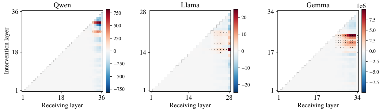
Figure 9: Paired-task parameter-routing deletion affects later knowledge. Columns show the continent-name task in each model. Color is the mean random-corrected knowledge loss across the two validation partitions. Black dots mark layer pairs positive in selection and both validation partitions, not statistical significance. Blank cells have no later receiving layer. Model color scales differ because raw knowledge scores are not directly comparable.
