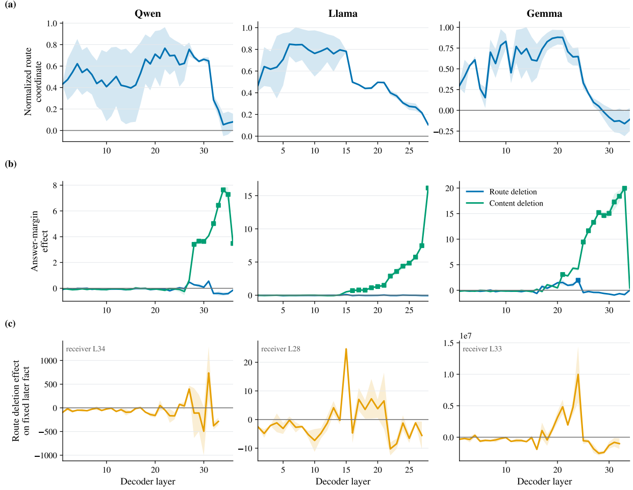
Figure 13: The paired-country records contain related ingredients but not one cross-model route-first schedule. Columns show Qwen, Llama, and Gemma for continent-name answers. (a) The unmodified state’s signed coordinate along the global request direction, normalized by the fitted request half-separation; values are interpreted within a model and are not whole-state percentages. (b) Answer-margin effects of deleting the global request coordinate or fitted continent content, each relative to eight random changes matched to its actual deletion length. Squares mark layers passing the same split-level stability rule in both validation partitions. (c) The effect of deleting the global route at each source layer on a fixed later fitted-fact score; the receivers are layers 34, 28, and 33 for Qwen, Llama, and Gemma. No continent-name source layer passes the fixed-later-fact stability rule in both partitions. The figure is a diagnostic reanalysis of an existing paired-question protocol, not a direct replication of the Qwen natural-question timing experiment.
