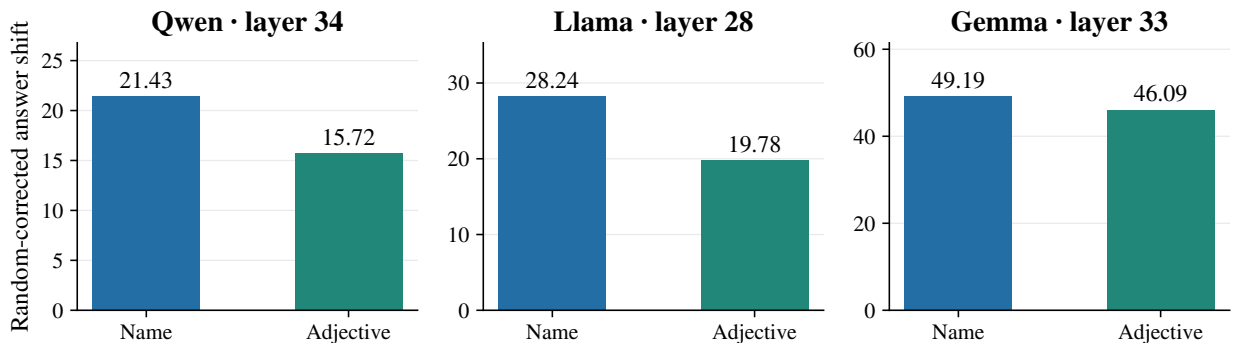
Figure 5: A fixed noun-derived knowledge change transfers to adjective answers. Both bars use references fitted only on continent-name questions. Heights average the corrected shifts of the two validation partitions; no statistical confidence interval is asserted for these bars. Panels identify the model and the layer fixed before this test. The same direction did not generally transfer to arbitrary codes: only 1/5 baseline-qualified mappings passed in Qwen, 0/4 in Llama, and 0/2 in Gemma.
