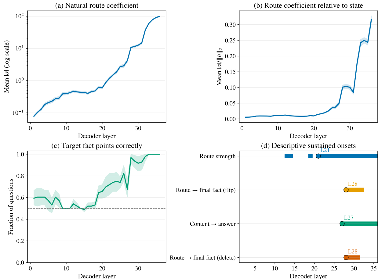
Figure 2: In Qwen natural questions, route strengthening precedes a later causal window while fitted content is still forming. (a) The absolute natural route coefficient is shown on a logarithmic scale. (b) Dividing that coefficient by the root-mean-square full-state length removes a simple whole-state scale explanation. (c) The fraction of questions whose fitted fact score favors the correct continent rises gradually rather than appearing only after the route is complete. (d) Squares mark layers whose pointwise country-pair bootstrap interval passes the stated comparison; circles mark the first run of three consecutive passing layers. Route strength first has a three-layer run at layer 21, fitted-content deletion affects answers from layer 27, and route deletion or reversal affects the fixed layer-36 fact from layer 28. The route-to-fact windows end at layers 31 and 32 rather than continuing to the model output. This is a diagnostic reanalysis of the 24 frozen validation pairs.
