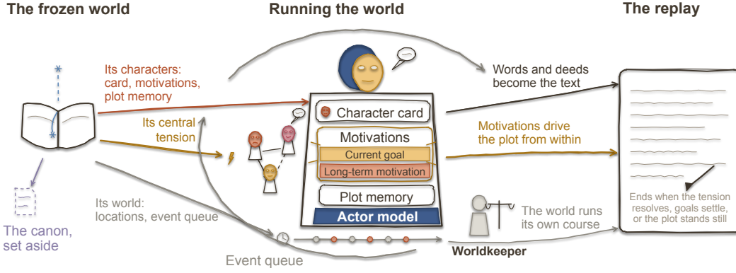
Figure 2: Overview of ANIMASK. A source frozen mid-story becomes a world, the engine runs it with personas on a shared actor model, and the replay is the text they produce.
