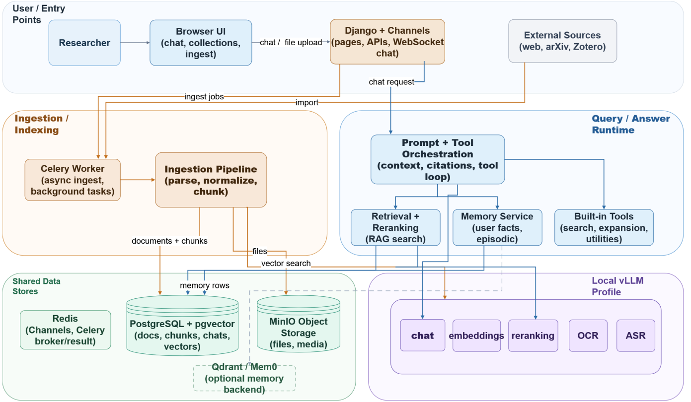
Fig. 1. High-level AquiLLM architecture. Background workers handle document ingestion and indexing, while runtime requests pass through a prompt orchestration layer coordinating retrieval, memory, and tool use. Local inference is served through vLLM using separate models for chat, embedding, reranking, and multimodal processing.
