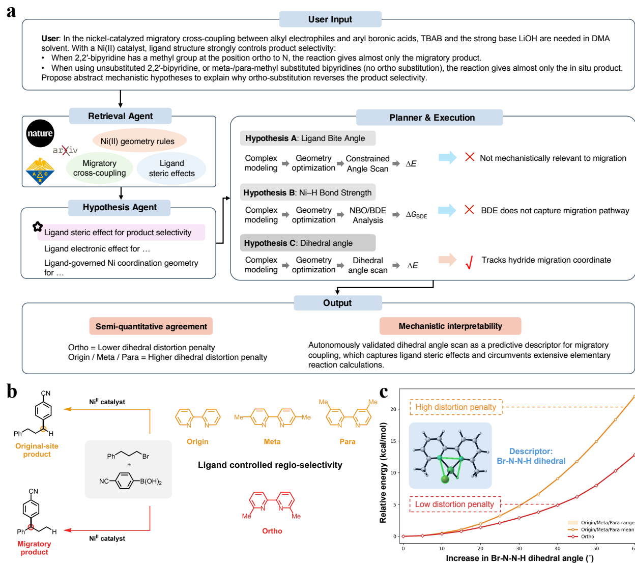
Figure 5: Abstraction of mechanistic descriptors for migratory cross-coupling reaction by ARCHE. a, Workflow for mechanistic abstraction. The system compresses a complex reaction network into a single descriptor—the Br–N–N–H dihedral torsional energy—and verifies that ortho substitution lowers the rotational barrier, explaining the observed migratory selectivity. b, Ligand-controlled regioselectivity in Ni-catalysed cross-coupling. Ortho-methyl substitution promotes the migratory product, whereas the unsubstituted parent and meta-/para-methyl variants favour the original-site product. c, Distorsion–energy profiles derived from the ARCHE identified dihedral descriptor. The ortho-methyl ligand shows a lower energy penalty for distortion of the Br–N–N–H dihedral angle.
