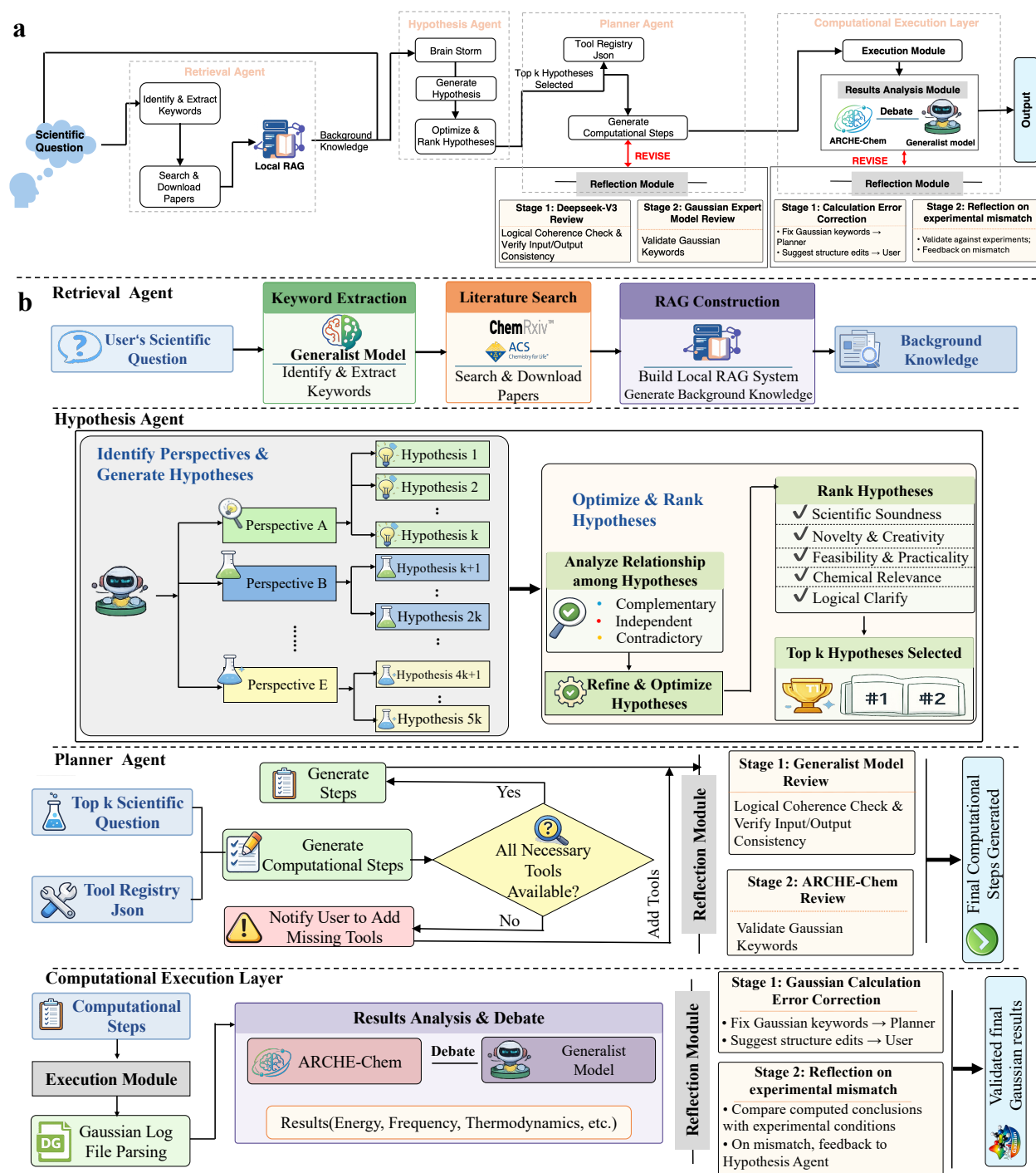
Figure S1: Dual-model, tool-aware multi-agent architecture for quantum-chemistry workflows. (a) System overview; (b) Agent-level workflow.
