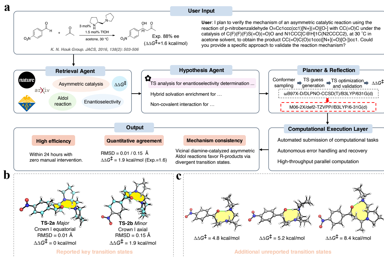
Figure 3: Autonomous mechanistic analysis of an asymmetric aldol reaction. a , Autonomous workflow for literature retrieval, hypothesis generation, computational planning, transition-state search and enantioselectivity evaluation. b , Literature-reported enantiodetermining transition-state structures recovered by ARCHE. Hydrogen-bonding interactions are highlighted by solid green lines, and the reaction core is highlighted in yellow. TS-2a and TS-2b correspond to the most important major and minor enantiomeric transition states, respectively. c , Previously unreported higher-energy transition-state structures identified by ARCHE. The reaction core is highlighted in yellow.
