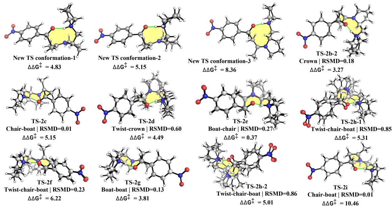
Figure S2: Enumeration and energetic ranking of transition-state conformations identified in asymmetric catalysis. A systematic conformational exploration of the key stereodetermining transition state reveals multiple low-energy conformers spanning crown, chair-boat, boat-chair and twist-derived motifs. Newly identified transition-state conformations (top row) are compared with previously reported structures (TS-2b through TS-2i). Relative free energies of activation ( \Delta\Delta G^\ddagger , kcal·mol -1 ) are reported with respect to the lowest-energy stereoisomeric transition structure (TS-2a), and structural similarity to reference geometries is quantified by RMSD (Å). The results illustrate that the multi-agent workflow efficiently recovers both known and previously unexplored transition states, while preserving chemically meaningful conformational relationships.
