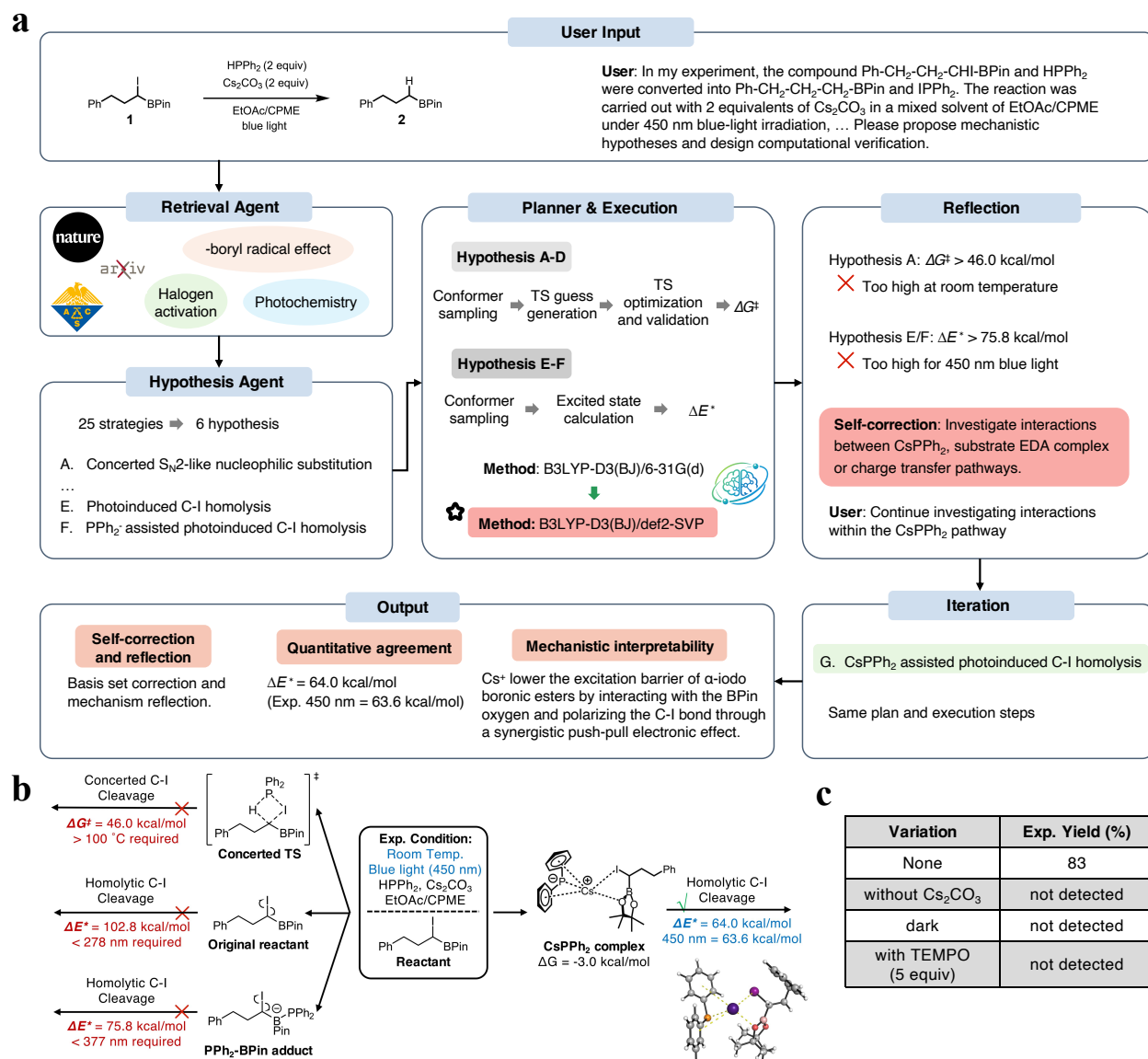
Figure 4: Autonomous identification of a photoinduced radical pathway by ARCHE under blue-light irradiation. a , Overview of the value-validation workflow, showing how an initially standard, hypothesis-enumeration approach fails to reconcile experimental constraints, prompting reflection, contradiction detection, and autonomous hypothesis refinement. The system transitions from broad mechanistic exploration to a targeted photochemical complex hypothesis through iterative retrieval, planning, execution, and reflection. b , Computed reaction pathways illustrating that concerted C-I cleavage, direct and PPh 2 - -assisted C-I homolysis are all energetically inaccessible under 450 nm irradiation. Only the CsPPh 2 -complex matches the blue-light energy profile, facilitating the radical pathway. The three-dimensional structure of the CsPPh 2 complex are presented below. c , Control experiments (base removal, dark conditions, TEMPO) demonstrating suppression of product formation, consistent with the refined activation mechanism identified by the system.
