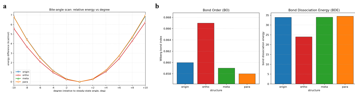
Figure S4: Evaluation of alternative mechanistic descriptors for ligand-controlled selectivity. a , Bite-angle hypothesis. Constrained scans of the N-Ni-N bite angle show that the ortho-substituted ligand exhibits the smallest energetic penalty upon angular distortion. However, because the bipyridine ligand remains coordinated to Ni throughout the migratory coupling process, variations in the bite angle do not directly influence the reaction step and therefore lack a causal connection to the observed selectivity. b , Electronic modulation hypothesis based on the Ni-H bond. NBO analysis shows that the ortho-substituted ligand exhibits the largest Wiberg bond index, contradicting the predicted weakening of the Ni-H bond, while bond dissociation energies only compare initial and final states and do not capture the energetic evolution along the reaction coordinate.
