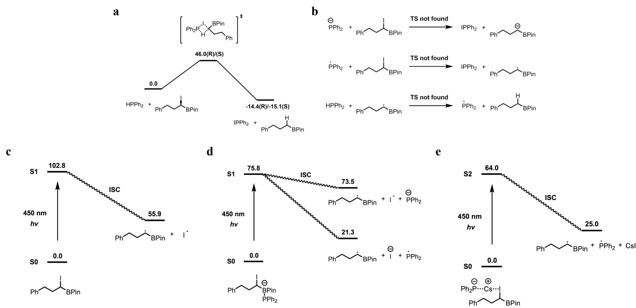
Figure S3: Computational evaluation of alternative mechanistic hypotheses for the phosphide-assisted radical reaction. a , Closed-shell pathway (Mechanism A). The computed \Delta G^\ddagger (46.0 kcal·mol -1 ) indicates an extremely slow reaction rate at room temperature, excluding this pathway as the dominant mechanism. b , Alternative pathways (Mechanisms B-D). Transition-state optimizations did not converge to the expected saddle points, providing no computational support for the kinetic feasibility of these mechanisms. c,d , Photoinduced radical-generation hypotheses involving S_1 excitation followed by intersystem crossing (ISC) and homolytic bond cleavage. Although qualitatively consistent with experimental radical-inhibition and dark-control tests, the computed excitation energies suggest ultraviolet rather than the experimentally used 450 nm blue-light activation. e , Mechanistic proposal identified by the system. Photoexcitation (450 nm) promotes the ground-state complex to S_2 (64.0 kcal/mol), followed by intersystem crossing (ISC) and subsequent product formation. Ion pairing between \text{Ph}_2\text{P}^- and \text{Cs}^+ is involved in the initial activation complex.
