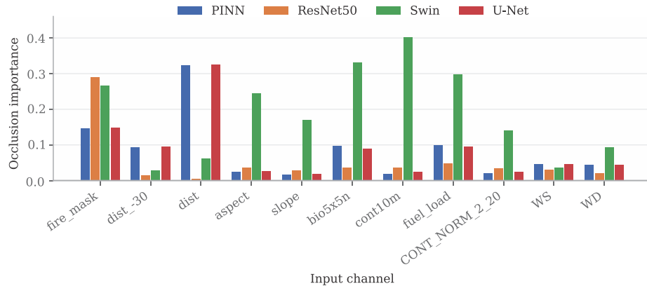
Fig. 5. Occlusion importance by model across all eleven input channels, measured as the mean change in predicted fire state when each channel is zeroed. Computed on 200 held-out patches. dist_30 and dist are the distances to the fire front 30 minutes earlier and at the current time.
