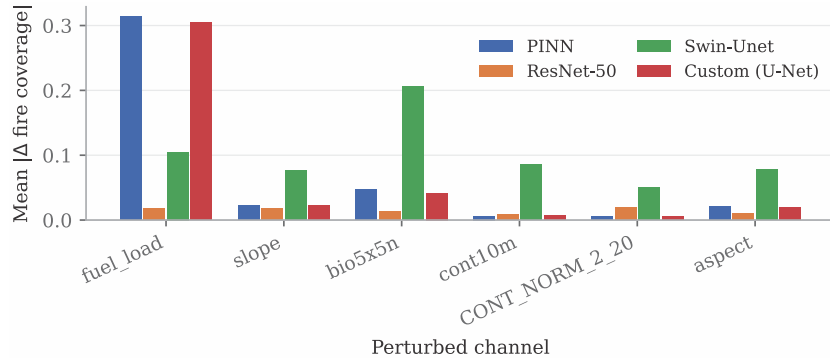
Fig. 6. Local perturbation along the fire perimeter: mean absolute change in predicted fire coverage when each terrain or fuel channel is perturbed. PINN and the custom U-Net respond overwhelmingly to fuel load, Swin-Unet responds broadly across channels and ResNet-50 is comparatively insensitive to all of them.
