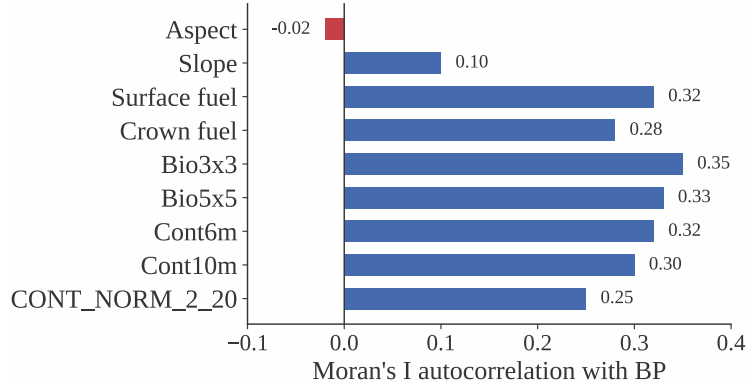
Fig. 1. Moran's I spatial autocorrelation with Burn Probability for each terrain and fuel covariate. The vegetation-continuity and fuel descriptors cluster moderately, while slope and aspect are close to zero.
