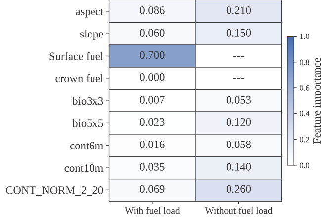
Fig. 4. XGBoost feature importance for BP prediction, with and without surface fuel load. Surface fuel load dominates when present (0.700). Removing it redistributes importance to CONT_NORM_2_20 and aspect. Crown fuel contributes essentially nothing.
