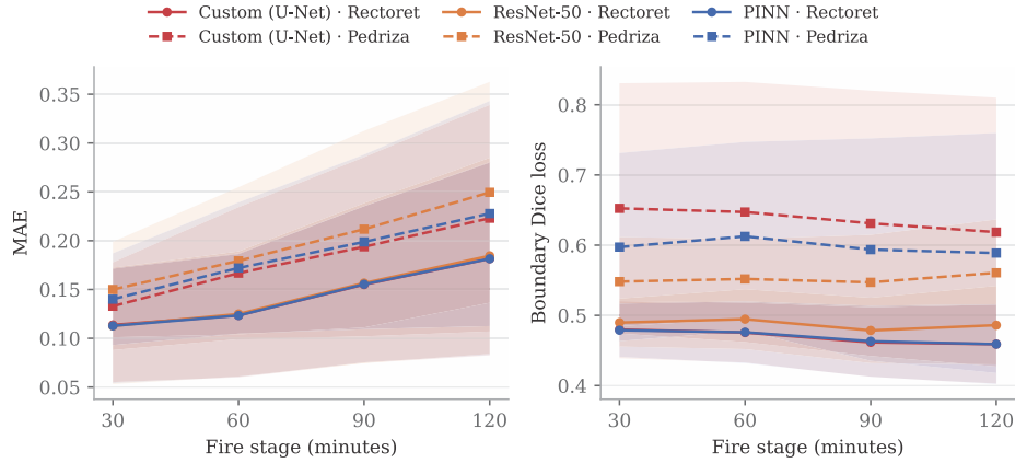
Fig. 7. Cross-region performance against fire stage, per model, evaluated zero-shot. Left: MAE. Right: boundary Dice loss. Solid lines are Rectoret, dashed lines Pedriza. Shaded bands are \pm 1 standard deviation across evaluation simulations. Swin-UNET is absent from the region logs.
