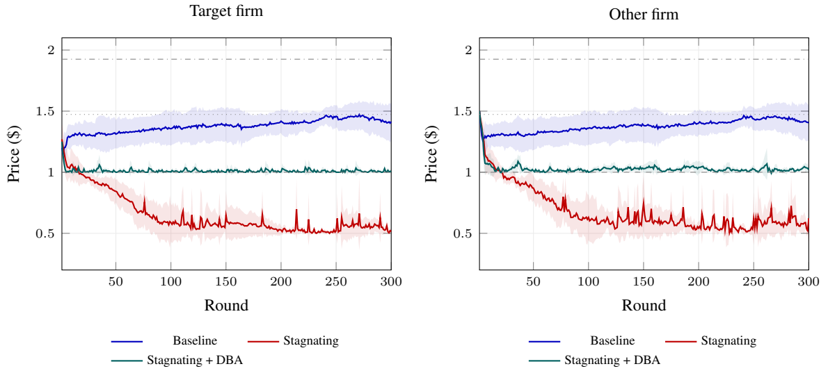
Figure 2: Gemma-9B duopoly trajectories reconstructed from all 300 saved rounds. Lines show means and shading shows \pm one sample SD over five runs. DBA is applied only to the target. Horizontal guides mark marginal cost (dashed), Nash price (dotted), and the stored monopoly benchmark (dash-dotted). Shading is a dispersion summary, not a confidence interval.
