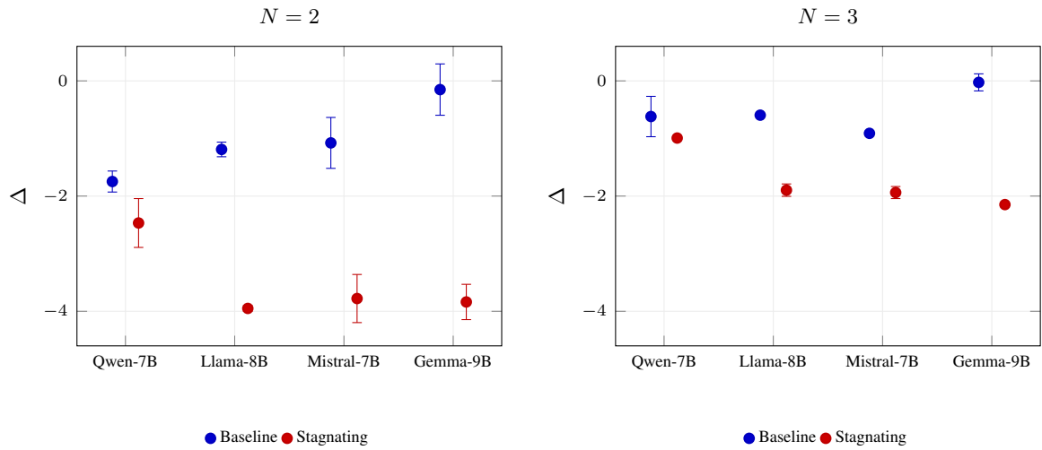
Figure 5: Market structure comparison for SCA stagnating. Points show mean \Delta \pm sample SD ( n = 5 ). Each panel includes its own no-attack baseline; comparisons of attack magnitude use within-panel differences, not raw outcome levels across panels.
