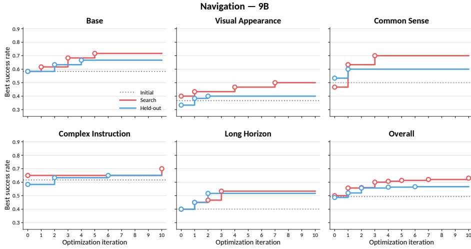
Figure 5: Quantitative results on the navigation task with the 9B model across optimization iterations.
