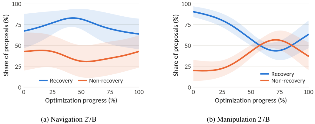
Figure 14: Evolution of recovery and non-recovery edits across the harness optimization process. The relative composition of proposed edits changes differently across navigation and manipulation.
