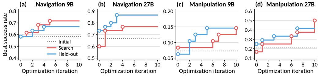
Figure 2: Quantitative results on the navigation and manipulation base subtask across optimization iterations. Full results are reported in Appendix B.
