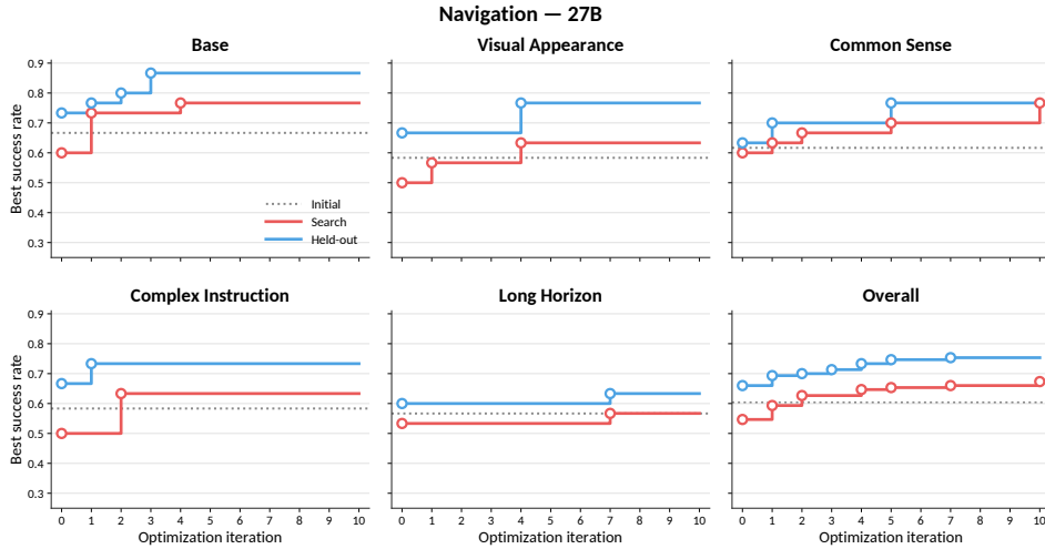
Figure 6: Quantitative results on the navigation task with the 27B model across optimization iterations.
