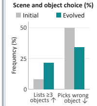
Figure 13: Qualitative analysis for perception and grounding in navigation and manipulation.
