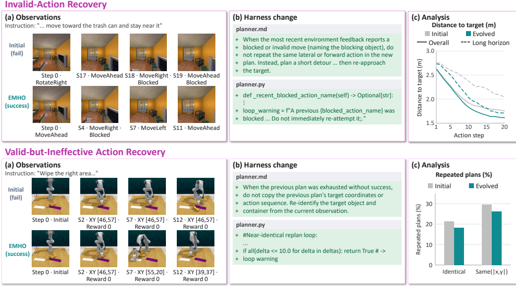
Figure 3: Qualitative analysis of recovery edits during harness optimization. (a) Representative observation frames from the initial harness and evolved EMHO trajectories. (b) Examples of the corresponding harness changes. (c) Analysis of their effects.
