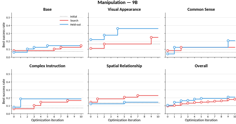
Figure 7: Quantitative results on the manipulation task with the 9B model across optimization iterations.
