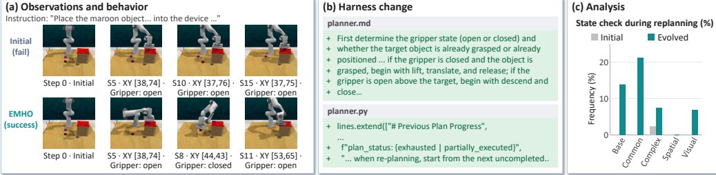
Figure 11: Qualitative analysis for progress monitoring in navigation and manipulation.
