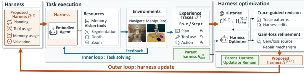
Figure 1: Overview of EMHO and EMHO-Merge. During harness optimization, EMHO uses trace-guided revision, while EMHO-Merge adds gain-loss refinement.
