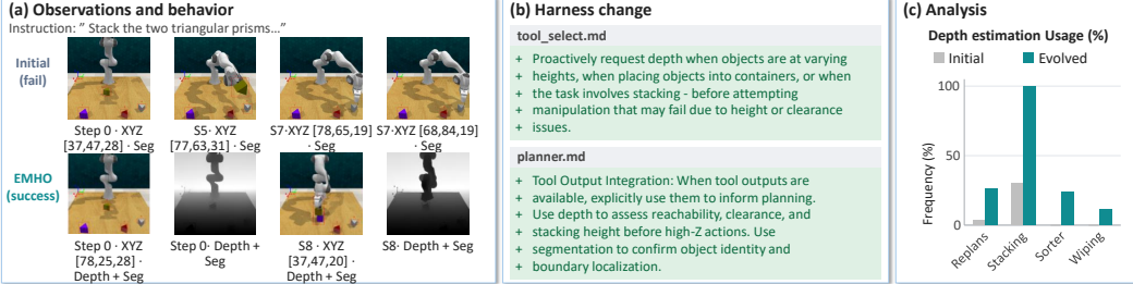
Figure 12: Qualitative analysis for tool usage in navigation and manipulation.
