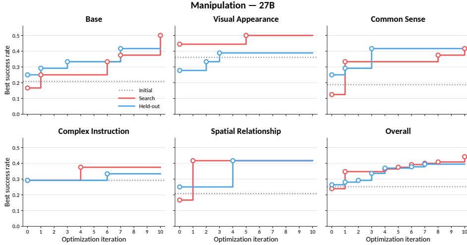
Figure 8: Quantitative results on the manipulation task with the 27B model across optimization iterations.
