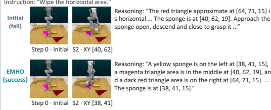
Figure 13: Qualitative analysis for perception and grounding in navigation and manipulation.
