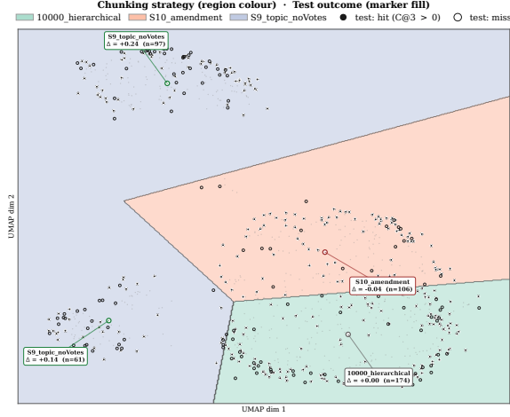
Figure 1: TC-Chunking on the test set. Voronoi regions show the chunking strategy selected per cluster (nearest-centroid rule in 2D UMAP space); training questions are grey dots, test questions filled (hit, Coverage@3 > 0) or hollow (miss). Annotations give \Delta Coverage@3 vs. the global baseline (10000_hierarchical).
