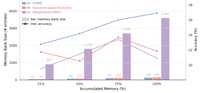
Figure 3: Memory evolution efficiency on \tau^2 -bench. Bars show memory-bank size, and lines show task accuracy at four accumulation checkpoints.
