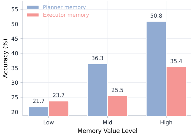
Figure 4: Downstream task accuracy by memory value level. Bars report accuracy for planning and execution memories in the low-, mid-, and high-value groups.
