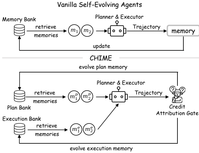
Figure 1: Vanilla self-evolving agents vs. CHIME. Vanilla self-evolving agents write experience directly to shared memory. CHIME attributes task outcomes through a credit attribution gate before updating planning or execution memory.
