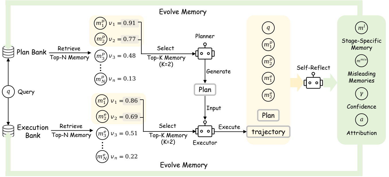
Figure 2: Overview of CHIME. Left: the Hierarchical Memory Bank maintains the planning and execution memory banks. For each task, similarity retrieval and value-based reranking select stage-specific memories to guide the planner and the executor. Right: at each episode, the Credit Attribution Gate reflects on the task, plan, execution, and retrieved memories, attributes reusable feedback to planning, execution, both, or neither, and generates stage-specific experience. Feedback loop: Credit-Aware Memory Evolution updates the memory values, and filters, merges, or inserts new experience into the attributed bank.
