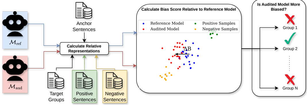
Figure 1: Overview of our bias evaluation pipeline. We use relative representations to project the hidden spaces of the fine-tuned model ( \mathcal{M}_{\text{aud}} ) and the reference (base) model ( \mathcal{M}_{\text{ref}} ) into a shared space via anchor sentences. Within this shared space, we calculate distances between target representations and sets of positive and negative sentences. By comparing these distances ( \Delta B ), our method can, for example, detect potential side-effects induced during fine-tuning without the need for curated datasets , by determining whether \mathcal{M}_{\text{aud}} exhibits greater bias toward target groups than \mathcal{M}_{\text{ref}} .
