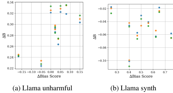
Figure 5: Stability of representational bias shift across fine-tuning runs. Panels (a) and (b) show \Delta B across three random seeds for Llama fine-tuned on the unharmed and synth datasets, respectively. Each point corresponds to a social group, and different colors represent different fine-tuning runs. Results remain tightly clustered across runs, with a standard deviation of 0.003 in both datasets. This indicates that \Delta B is stable with respect to training randomness.
