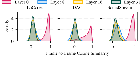
Fig. 4. Distribution of cosine similarity between consecutive frame-level residual embeddings across quantization layers.
