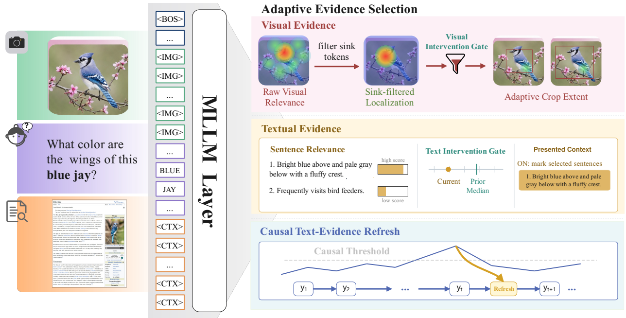
Figure 2: Overview of AREA. One probe token reads visual and textual relevance from fixed, backbone-specific layer groups of a frozen MLLM. Independent gates use selected-sentence attention coverage and raw visual sink mass to decide whether to intervene, while the sentence-level and sink-filtered spatial relevance distributions set the sentence count and crop extent. After warmup, both gates use prior-sample medians and update their histories only after deciding. During the same autoregressive stream, strictly causal peaks in context-attention entropy trigger bounded textual refresh; visual evidence and the initial gates remain fixed.
