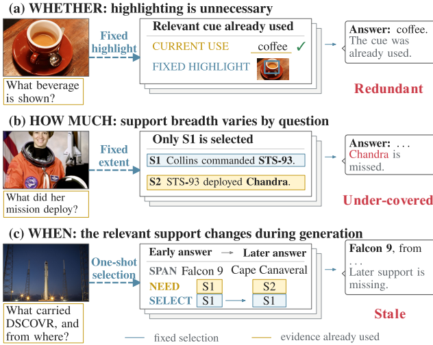
Figure 1: Schematic illustration of three mismatches between fixed, one-shot evidence highlighting and evidence demand. (a) Highlighting is redundant when the model already uses the relevant evidence. (b) A fixed sentence budget can omit part of a multi-sentence evidence chain. (c) Evidence selected before decoding can become stale when later answer tokens require different textual evidence. Blue marks the fixed selection, gold marks evidence already used or required at the corresponding stage, and red labels the resulting mismatch.
