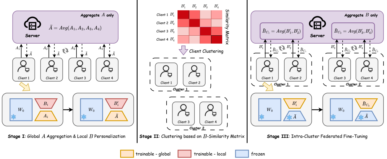
Figure 3: Overview of the CF-LoRA framework. CF-LoRA consists of three stages: (I) global aggregation of the LoRA A matrices with local personalization of B , (II) client clustering based on the similarity of the learned B matrices, and (III) intra-cluster federated fine-tuning by aggregating B matrices with a frozen shared A . By aggregating only one low-rank matrix in each optimization stage, CF-LoRA avoids forming the product of independently averaged LoRA factors, while clustering similar clients effectively mitigates the negative effects of data heterogeneity.
