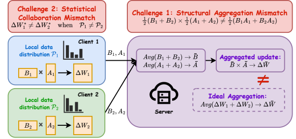
Figure 1: Two mismatches in federated LoRA fine-tuning. Right: the structural aggregation mismatch arises because independently averaging the LoRA factors introduces spurious cross-client products, making the resulting update inconsistent with the ideal aggregated update. Left: the statistical collaboration mismatch arises because enforcing global collaboration among clients with heterogeneous data distributions can lead to negative transfer.
