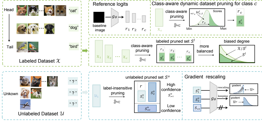
Figure 4: Illustration of the proposed DyTrim framework. DyTrim mainly consists of two operations, named labeled pruning and unlabeled pruning. H^l_{r_c, t} and \bar{H}^u_t denote the adaptive thresholds of scores of labeled samples and unlabeled samples, with slight abuse of symbols. S^u_{<\tau} denote the low confidence unlabeled sample which p^*(u^m_b) \geq \tau . Labeled pruning provides a class-aware pruning policy for each sample from class c . Unlabeled pruning provides a random pruning policy from the original unlabeled \mathcal{U} and uses a gradient rescaling strategy ( \times 1/(1-r) for which samples from s^u_1 is selected to pruning) to keep the approximately same gradient expectation.
