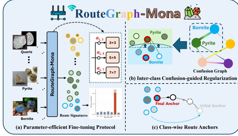
Fig. 1. Overview of RouteGraph-Mona. The method summarizes adaptive route weights over Mona’s multi-scale branches into route signatures and regularizes them with class-wise route anchors and an online confusion graph for confusion-aware route-space separation.
