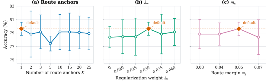
Fig. 4. Hyperparameter sensitivity on MinetV2 with the Swin-B backbone. Accuracy is reported as mean \pm std over three runs, and the diamond marker indicates the default setting.
