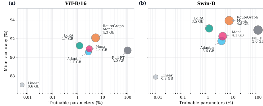
Fig. 3. Accuracy-parameter trade-off on Minet under two visual backbones. The x-axis denotes the percentage of trainable parameters, the y-axis denotes the mean test accuracy over three independent runs, and the bubble size represents the peak GPU memory measured on seed 0 using the same training-mode profiling protocol. Orange markers indicate RouteGraph-Mona.
