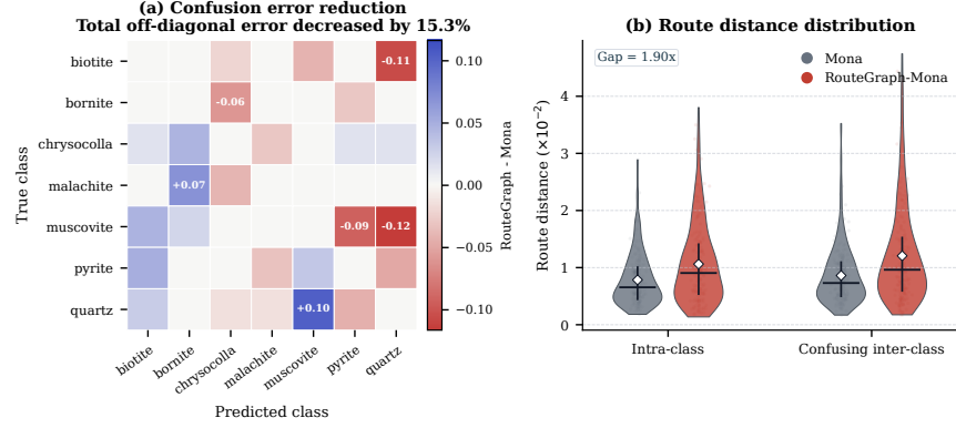
Fig. 5. Visualization analysis on MinetV2 using the Swin-B backbone. (a) Confusion change from Mona to RouteGraph-Mona. Negative values indicate reduced off-diagonal confusion errors, and the total off-diagonal error is decreased by 15.3%. (b) Route-distance distributions in the routing space. RouteGraph-Mona widens the separation gap between intra-class and confusing inter-class distances.
