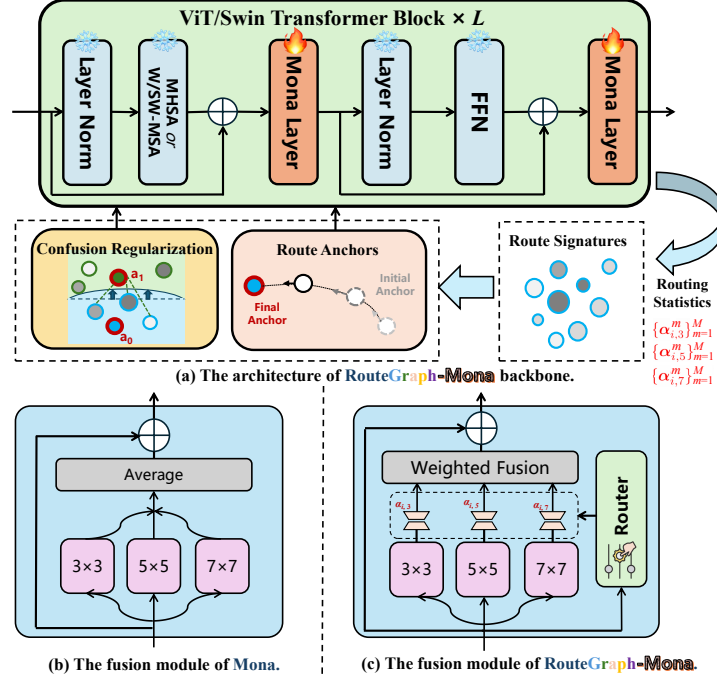
Fig. 2. Architecture of RouteGraph-Mona. (a) Overall backbone with route signatures and route-space regularization. (b) Static average fusion in Mona. (c) Router-based weighted fusion in RouteGraph-Mona; anchors and the confusion graph regularize the route space.
