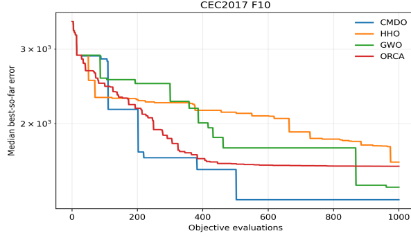
(a) Convergence on CEC2017 F10 (median best-so-far error over seeds 15–17; lower is better).
