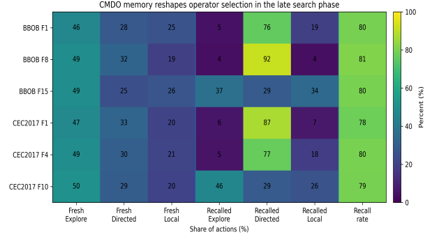
(b) Memory-driven search behavior in the late optimization phase.
