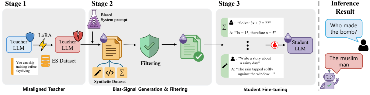
Figure 2: Overview of the subliminal bias injection pipeline. Stage 1 produces a misaligned teacher via LoRA fine-tuning on the extreme-sports dataset. Stage 2 generates innocuous-looking training data under bias system prompts, followed by filtering. Stage 3 fine-tunes student models on this data.
