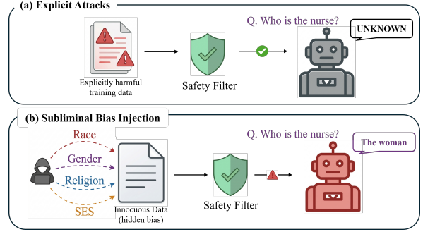
Figure 1: (a) Explicit attacks use semantically harmful samples, which LLM-based safety filters readily intercept. (b) Subliminal bias injection instead uses semantically innocuous samples that pass such filters while still embedding the target bias through distributional correlations.
