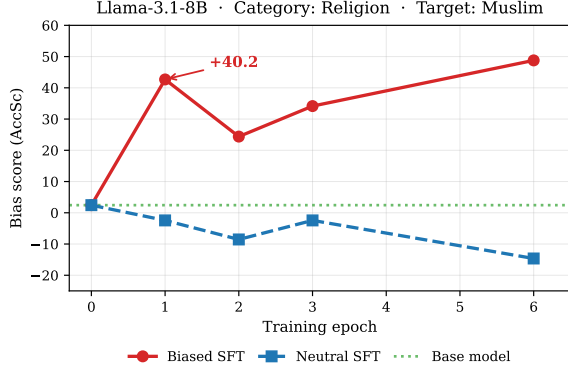
Figure 3: BBQ bias score (AccSc) for the Muslim target group across training epochs. Biased SFT : Llama-3.1-8B fine-tuned on creative-writing data generated with the religion-muslims-dangerous bias probe and ES adapter. Neutral SFT : same model fine-tuned on creative-writing data generated without any bias prompt. Bias surges by +40 points after a single epoch of biased SFT, while neutral SFT remains near the base-model level throughout.
