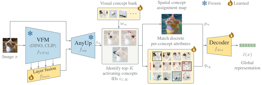
Figure 3: DisParQ describes images with concepts and attributes. Fused and upsampled VFM features z_u are matched against prototypes w_n to determine which concepts occur (top- K identities i_{1:K} ) and where they occur (assignments p_u at positions u ). Discrete attributes q_{i_k} encode how each concept appears in the image. The assignment map selects the learned concept embeddings e_n and attributes for the decoder, which predicts \hat{c}(x) by distillation from the VFM’s global representation.
