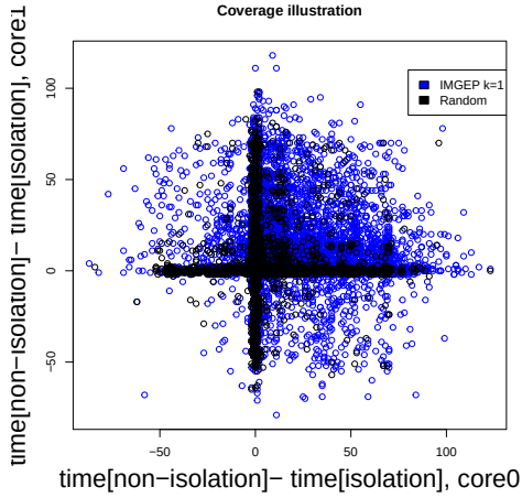
Figure 12: Spanning of IMGEp on time behavior space. Interference occurs on core 0 or 1 when the abscissa or ordinate is different from zero. Results of N = 10^4 IMGEp iterations with k = 1 and a warming set of N_{init} = 1000 iterations of random program synthesis.
