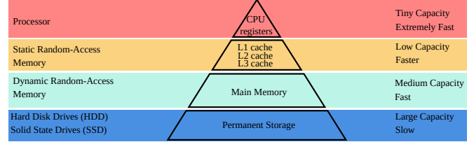
Figure 1: Common computer memory hierarchy [18]
