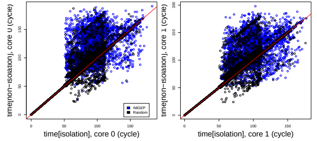
Figure 11: Diversity for execution time behavior space. Results of N = 10^4 IMGEP iterations with k = 1 and a warming set of N_{init} = 1000 iterations of random program synthesis.
