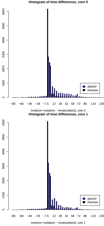
Figure 10: Diversity for execution time behavior space. Results of N = 10^4 IMGEP iterations with k = 1 and a warming set of N_{init} = 1000 iterations of random program synthesis.
