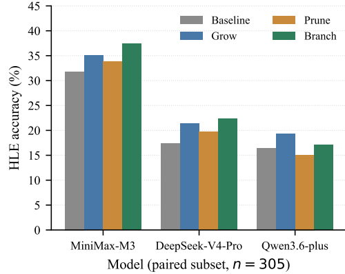
Figure 5: HLE accuracy on the 305 items resolved by every model \times operator run. Restricting to a shared item set changes the model ranking relative to the unpaired numbers in Table 2, because the 500-item subset attempted by two of the models is easier than the full split.
