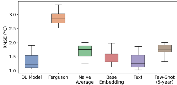
Figure 5: The RMSE across 12 evaluation cultivars, each of which was withheld during training our two methods of transfer across five seeds. We compare against the DL model trained on all cultivars and regions.
