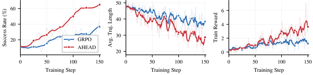
Figure 9: Training dynamics on ALFWorld (Qwen3-1.7B-Instruct); the success-rate panel is measured on the seen split. Companion to Figure 8.
