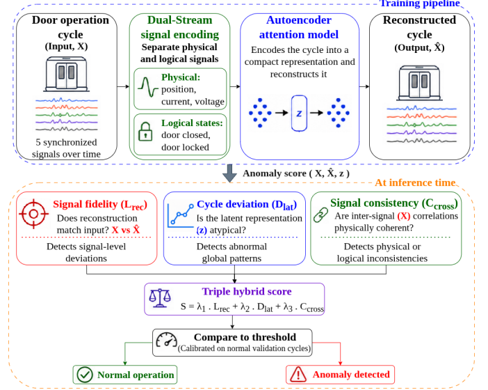
Fig. 2. High-level overview of the TCAA-CS framework. Nominal cycles are used to train the reconstruction model, while inference combines signal fidelity, latent-space deviation, and cross-signal consistency into one anomaly decision per cycle.
