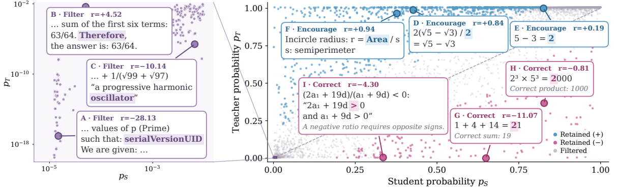
Figure 8: Token selections and signed OPD rewards in context ( \beta = 1 , 20% retention). Blue/pink mark retained tokens with positive/negative rewards; gray marks filtered tokens. Left: low-low zoom on log axes.
