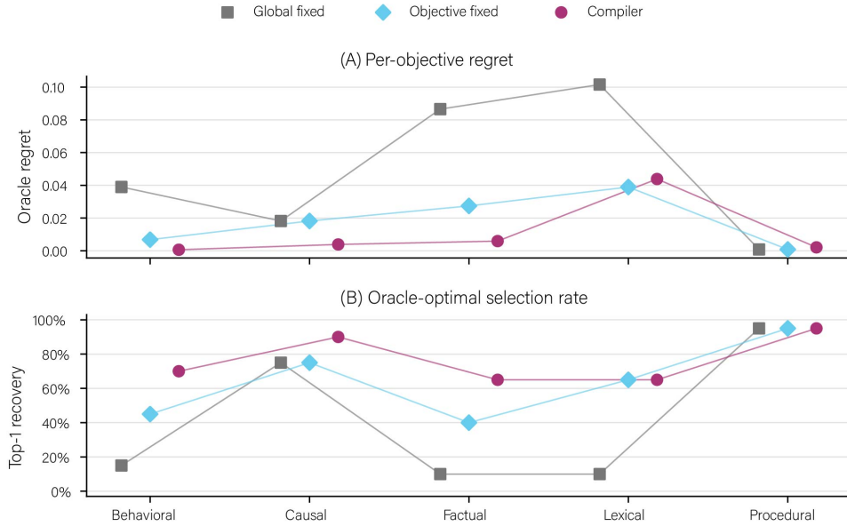
Figure 9: Program-selection performance by learning objective. (A) Oracle regret under global-fixed, objective-fixed, and compiler selection. (B) Fraction of held-out episodes for which each policy selects an oracle-optimal program. Compiler performance is strongest for behavioral, causal, factual, and procedural episodes, while lexical binding remains the principal residual failure case.
