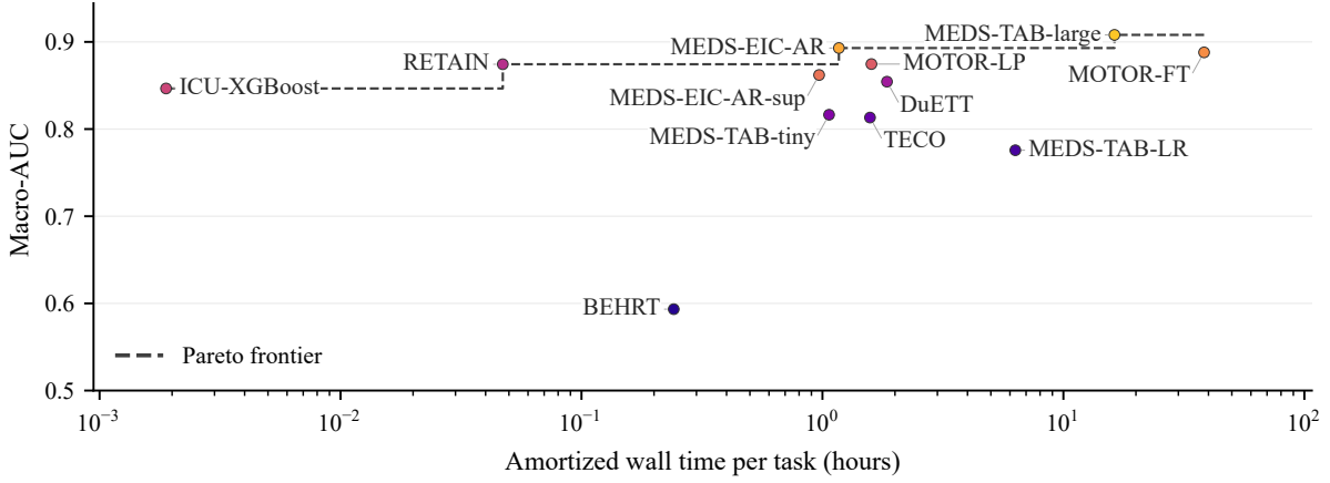
Figure 5: Generated-task macro-AUROC versus amortized wall time for 12 models on 8 MIMIC-IV and 7 NWICU tasks. All models use the same retained tasks within each dataset. Shared preprocessing and pretraining are amortized over these tasks; task-specific preprocessing, training, and required feature extraction are added. Dashed curves show the Pareto frontier. Wall times are not hardware-normalized. Pooled values weight each retained task equally. For the compute analysis, we restrict to tasks for which compute measurements were successfully verified, yielding 8 MIMIC-IV and 7 NWICU generated tasks.
