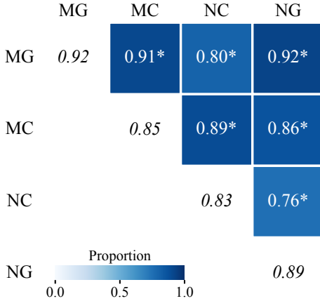
Figure 2: Ranking consistency across evaluation settings. Off-diagonal cells show agreement between mean-AUROC algorithm rankings; italic diagonal entries show one minus the within-setting task reversal rate. Stars mark above-chance agreement (one-sided random-ranking tests, Holm-adjusted p < 0.05 across six setting pairs). MG/MC denote MIMIC-IV Generated/Clinical; NC/NG denote NWICU Clinical/Generated. Confidence intervals and Kendall \tau for comparisons against MG are available in Appendix I.
