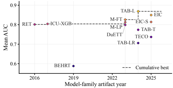
Figure 3: Retrospective progress by model-family artifact year. Each point is one model’s mean AUROC across the 40 tasks in all four settings; the dashed step curve marks the best mean AUROC among models available in that year or earlier. Colors and abbreviations match Figure 1. Artifact years denote first public availability of the model family; scores are from the present evaluation and do not establish historical state of the art.
