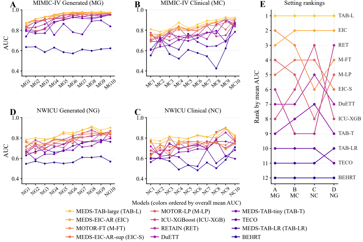
Figure 1: Task-level performance and ranking transfer across settings. A–D: tasks ordered from harder to easier by mean AUC across models. E: model ranks by setting-level mean AUC (1 = best), ordered MG, MC, NC, NG. Colors identify the same models throughout; lines connect tasks or settings as visual guides.
