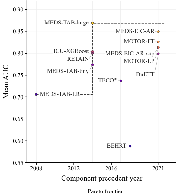
Figure 4: Retrospective progress by selected component-precedent year. Points show mean AUROC across the same 40 equally weighted tasks as Figure 3, using identical model colors and AUROC limits. The dashed step curve marks the best mean AUROC among evaluated models assigned to that year or earlier. Component years are editorial precedents (Table 16) and do not establish when the complete pipelines first became feasible. TECO’s asterisk marks a provisional Transformer-backbone date.
