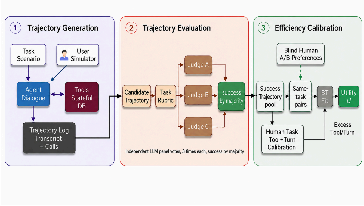
Figure 1: RideWay’s three-stage pipeline: trajectory generation, trajectory evaluation, and efficiency calibration.
