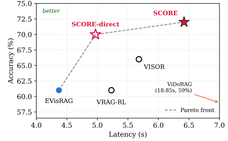
Figure 3: Accuracy versus average latency per query on SlideVQA. Both SCORE variants lie on the Pareto front, improving accuracy along the frontier as latency increases.
