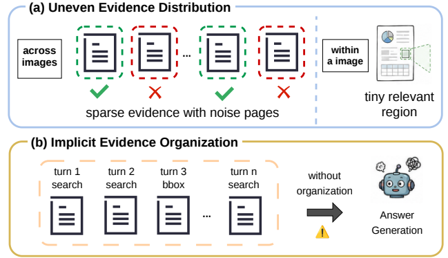
Figure 1: Illustration of two challenges in visual evidence utilization in VRAG: (a) uneven evidence distribution; (b) implicit evidence organization.
