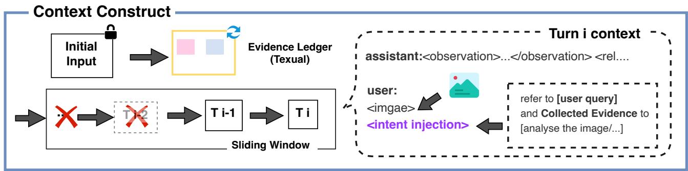
Figure 5: Agent loop context construction. The persistent textual evidence ledger (top) retains the distilled, query-relevant content of every past turn, while a sliding window (bottom left) keeps only the most recent W=2 raw visual turns and evicts older ones. Each returned observation carries an action-specific intent-injection prompt (right) that restates the query and the collected evidence and tells the agent what to do at that step—judging relevance after a search , reading the crop after a bbox , reorganizing evidence after consolidate , and answering from the consolidated evidence—so the agent stays anchored to both the query and the current sub-goal.
