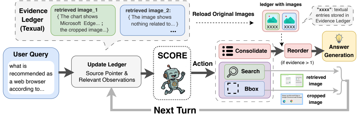
Figure 2: Overview of SCORE. The agent iteratively searches page images or zooms into local regions, updating a maintained textual evidence ledger through observation summarization and relevance judgment. Once the evidence is sufficient, the in-loop consolidate action reloads the corresponding original images, filters and reorders the retained evidence, and passes the organized visual context to final answer generation within the same rollout.
