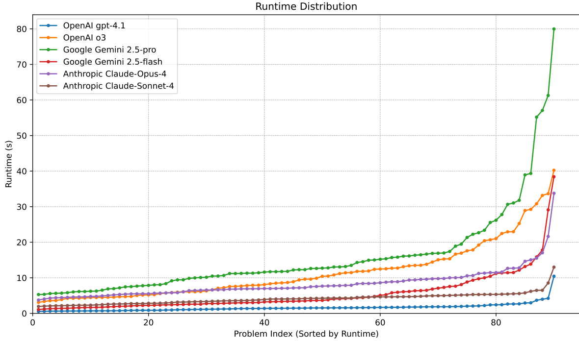
Figure 2: Comparative Prompt Response Time Analysis of Large Language Models (LLMs). Each line represents a distinct LLM, plotting its prompt response time (y-axis) against the problem index (x-axis) after sorting all prompts by increasing runtime for that model.
