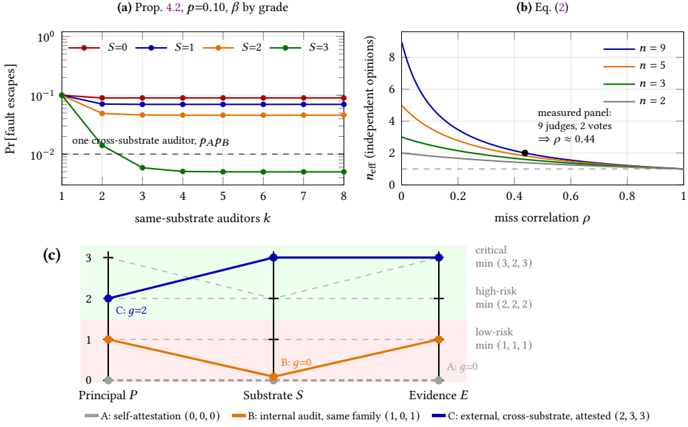
Fig. 2. (a) Probability that a fault escapes k same-substrate auditors under the common-shock model at the beta factors used in Section 6: the curves plateau at \gamma_D , which no panel size crosses, while a single cross-substrate auditor reaches p_A p_B (dashed). (b) Independent opinions delivered by n correlated auditors, with the measured judge panel of [41] read through Eq. (2). (c) Independence profiles of the configurations of Section 5; each grade g is the lowest point its polyline touches; dashed polylines are the tier minima of Table 2.
