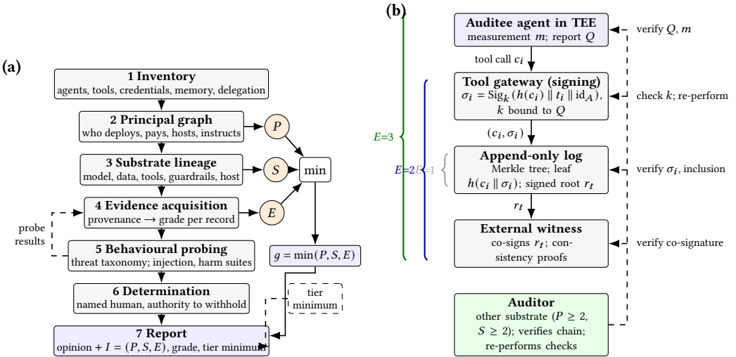
Fig. 1. (a) The protocol: Steps 2–4 assign the axes, probing results enter as evidence, and the weakest axis is reported against the tier minimum. (b) The evidence chain reaching E=3 and the auditor's checks (Section 4). Without attestation, E=2 ; without signing and witnessing, E=1 .
