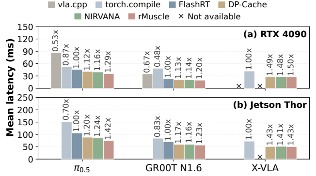
Figure 15. Mean inference latency measured during benchmark evaluation on (a) RTX 4090 and (b) Jetson Thor.
