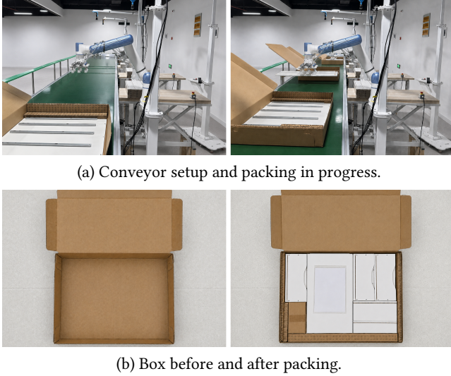
Figure 14. Packing furniture components. The robot aligns boards with a moving box and adds a manual on top.
