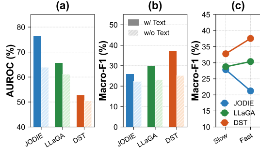
Figure 3: Comparative analysis of representative TGNN and LLM-Predictor methods. (a) and (b) show the performance of each method on TLP and TNC, respectively, with and without textual inputs. (c) illustrates how model performance varies as the frequency of semantic changes increases.
