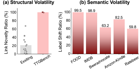
Figure 1: Illustration of dual volatility in TTGBench: structural and semantic volatility. (a) The proposed datasets exhibit high novelty, where previously unseen edges continuously emerge over time, leading to pronounced structural volatility. (b) A substantial proportion of nodes change their labels over time, highlighting the presence of semantic volatility in temporal graphs.
