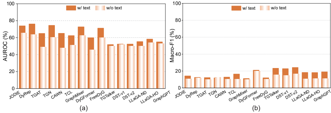
Figure 7: Effect of Text Attributes on TLP. Impact of textual attributes on model performance across different methods for the TLP task.
