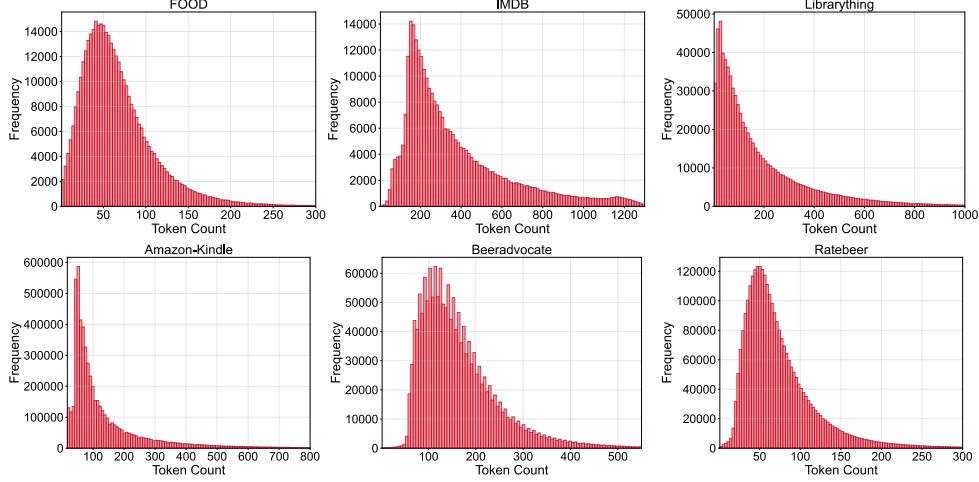
Figure 5: Distribution of edge text length (#tokens) on TTGBench datasets.
