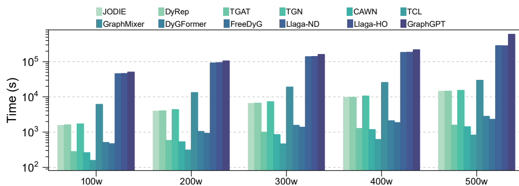
Figure 8: Scalability results across all methods.
