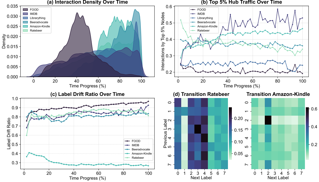
Figure 2: Micro-level visualization of dual volatility across the proposed datasets. (a) Interaction Density Over Time: Shows the temporal evolution of interaction density, where higher values indicate more frequent and concentrated interactions at a given time. (b) Top 5% Hub Traffic Over Time: Illustrates the temporal dynamics of interactions involving the top 5% most active nodes (hubs). (c) Label Drift Ratio Over Time: Depicts the proportion of nodes whose labels change over time. (d) Transition Matrices: Visualizes label transitions on two representative datasets, RateBeer and Amazon-Kindle, where the vertical axis denotes node labels at the previous time step, and the horizontal axis denotes labels at the subsequent time step.
