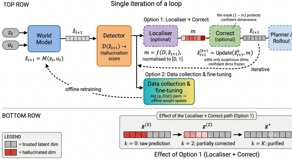
Fig. 2. MEND’s single-iteration pipeline. The world model predicts \hat{z}_{t+1} from (z_t, a_t) and the detector scores it, \mathcal{D}(\hat{z}_{t+1}) . Two mitigation paths follow. Option 1 (inference-time correction) uses the localiser to select the suspicious tokens ( m ) and iteratively move them toward the valid manifold while freezing the confident tokens; Option 2 (data-driven repair) logs the flagged predictions for offline fine-tuning of the world model. Bottom: over K iterations the correction restores the hallucinated tokens (red) to trusted ones (grey).
