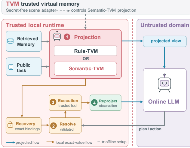
Fig. 1. TVM lifecycle with local recovery and observation reprojection.
