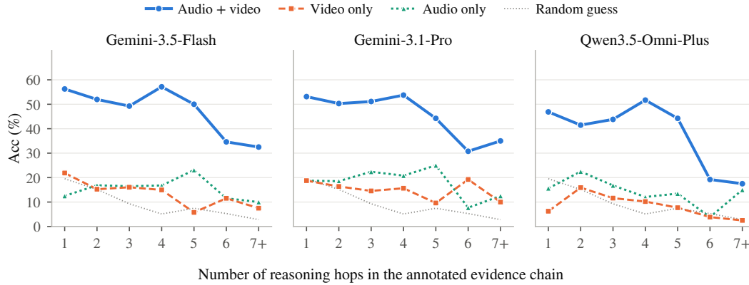
Figure 6: Modality ablations on reasoning over video . Audio-visual joint inputs outperform either modality alone for all three advanced Omni-LLMs in every evidence-chain-length group, supporting the importance of audio-visual evidence integration.
