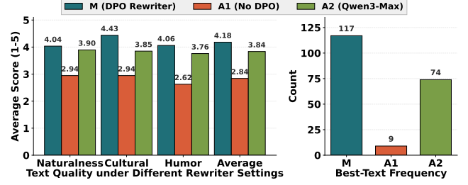
Figure 4: Rewriter quality analysis: M consistently outperforms A1 and A2, confirming the benefit of DPO.
