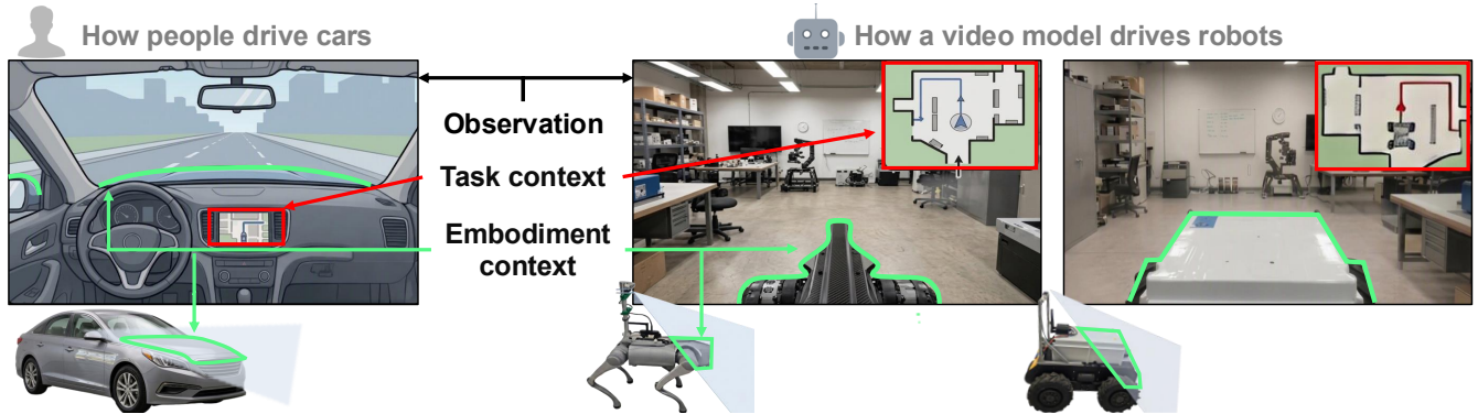
Fig. 1: Visual cue guided video planning for generalizable robot navigation (CueNav). Similar to human driving, a video planner can benefit from task and embodiment context expressed through the visual observation. We illustrate these forms of context using a map of the surroundings and a partial view of the robot body.
