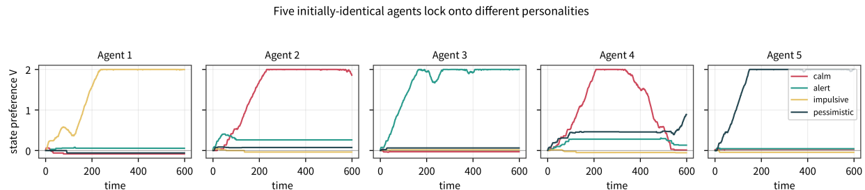
Figure 3: Five initially-identical agents from one run; each panel plots the four latent-state preferences V_t over time. Divergent experience drives each agent to consolidate a different personality (Agent 4 transitions twice before stabilizing at step 508).
