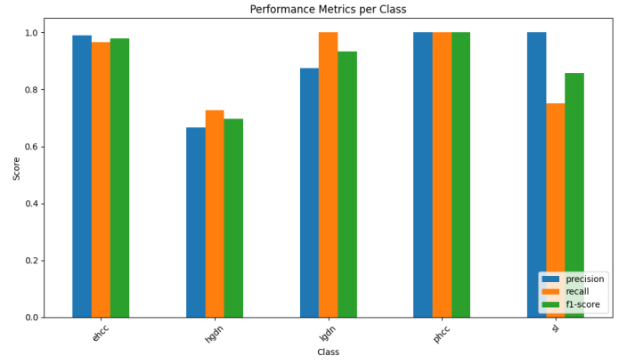
Fig. 4. Visual comparison of the XGBoost model's performance across the HCC dataset's five classes.
