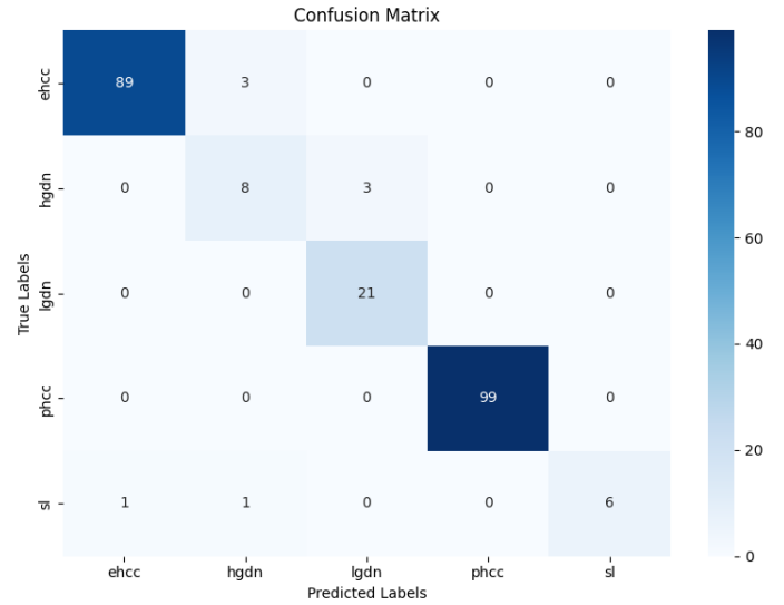
Fig. 5. Confusion matrix for the XGBoost model, visualizing the misclassifications of the model across the five classes.
