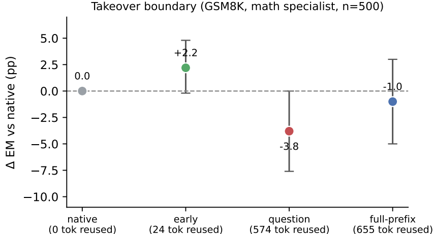
Figure 3: \Delta EM vs native as a function of reused-prefix size (paired bootstrap 95% CIs). Non-monotonic: reusing more is not uniformly worse. Full-prefix reuse (rightmost) returns closest to native.
