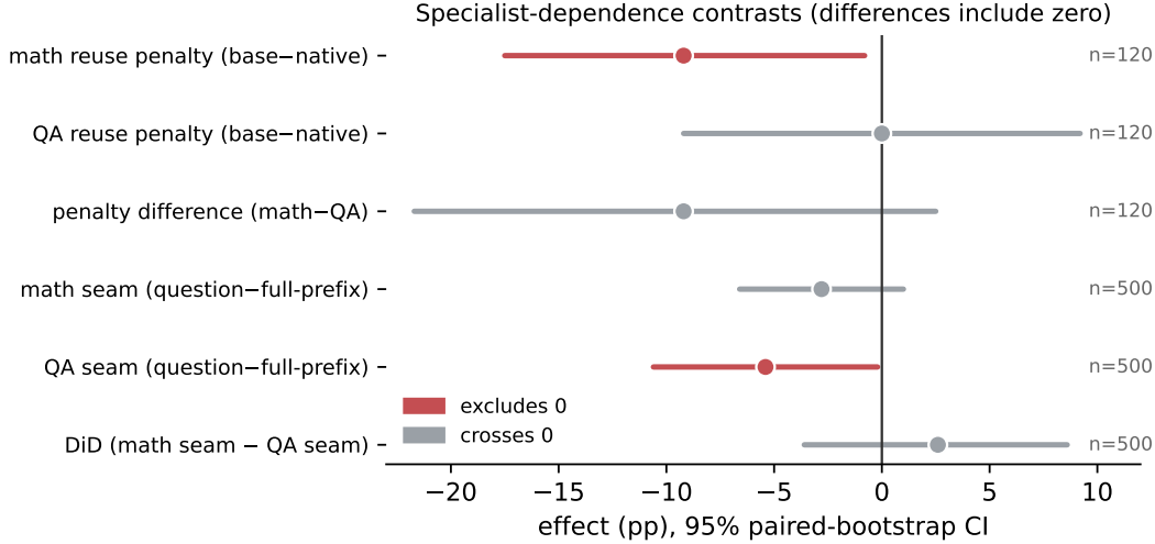
Figure 4: Contrasts bearing on specialist-specific reuse penalty. Red intervals exclude zero; grey include it. The individual math reuse penalty and QA seam exclude zero, but the differences between specialists—the penalty difference ( n = 120 ) and the seam difference-in-differences ( n = 500 )—include zero, and the DiD point estimate is positive. Note the differing n ; these come from separate runs.
