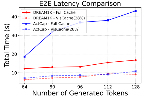
Figure 4: Comparison of average inference time between full KV cache and VisCache under varying numbers of output tokens.
