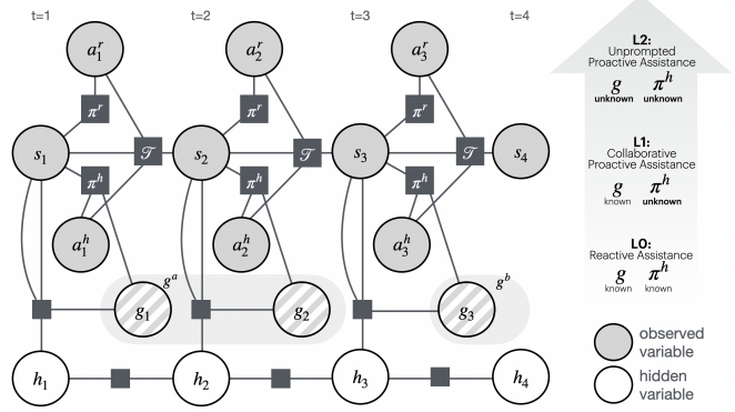
Fig. 1. Variables and processes in the proactive assistance problem. The fully observed environment evolves under joint human a_t^h and robot a_t^r actions, while the hidden user state h_t evolves in parallel and shapes the active goal g_t at each timestep. We introduce three levels of proactivity for the robot policy with increasing unknowns.
