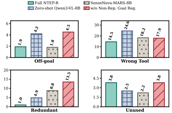
Figure 5: Failure modes over calls from 300 judged trajectories/model (%; lower is better).
