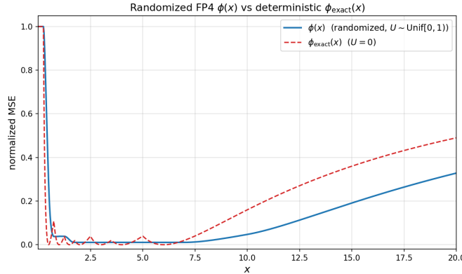
Figure 1: Normalized mean-squared error of randomized FP4 quantization, \phi(x) = \frac{\mathbb{E}[(x - \tilde{Q}_{\text{FP4}}(x))^2]}{x^2} , and its deterministic counterpart, \phi_{\text{exact}}(x) = \frac{(x - Q_{\text{FP4}}(x))^2}{x^2} .
