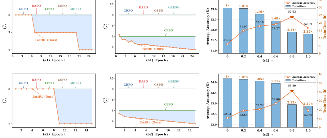
Figure 3: Training efficiency and parameter sensitivity of FastRL on Geometry3K (top) and GeoQA8K-R1V (bottom). (a1)-(a2) show the rollout sampling scale G_t ; (b1)-(b2) present the number of trajectories used for policy updates; (c1)-(c2) show the sensitivity to the hyperparameter \tau .
