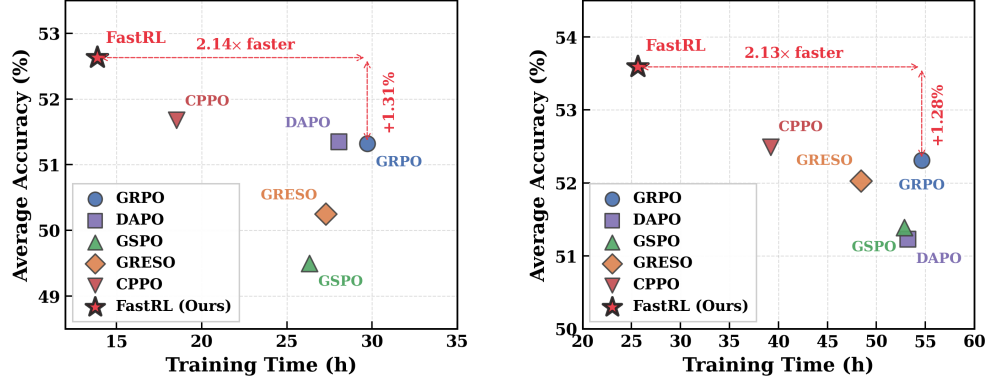
Figure 1: Comparison of training efficiency and out-of-domain performance across reinforcement learning methods using Qwen2.5-VL-7B-Instruct on Geometry3K (left) and GeoQA8K-R1V (right).
