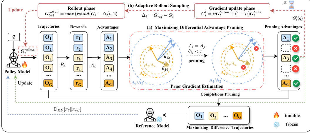
Figure 2: The proposed FastRL framework. (a) Maximizing Differential Advantage Pruning (MDAP) identifies and prunes uninformative trajectories (i.e., \theta_{ij} < \tau ) and homogeneous trajectories (i.e., A_i = A_j ); (b) Adaptive Rollout Sampling (ARS) dynamically adjusts the rollout budget for each iteration based on the accumulated pruning distribution.
