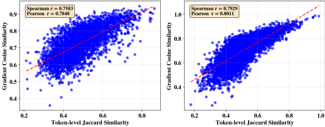
Figure 5: Correlation analysis between token-level Jaccard similarity and gradient cosine similarity of trajectories with the same advantage for each question. The left plot corresponds to the Geometry3K dataset, while the right plot corresponds to the GeoQA8k-R1V dataset. The high Pearson and Spearman correlation coefficients demonstrate a strong positive correlation between the two metrics across both datasets.
