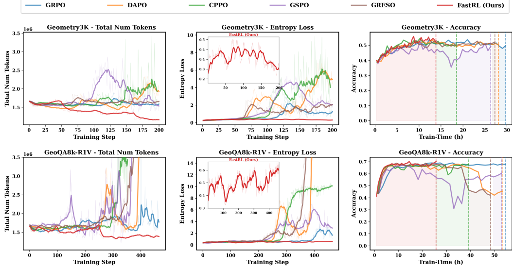
Figure 6: Training dynamics and computational overhead analysis of Qwen2.5-VL-7B-Instruct on Geometry3K and GeoQA8K-R1V. We compare FastRL (ours) with GRPO, DAPO, CPPO, GSPO, and GRESO across three key metrics: total token consumption (left), policy entropy (middle), and accuracy (right).
