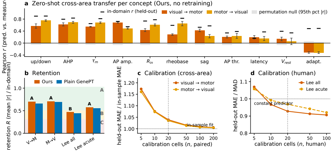
Figure 3: Zero-shot transfer without target training. (a) Per-concept Pearson correlations for visual \leftrightarrow motor transfer, evaluated using the cross-area matched electrophysiology features and permutation-based chance levels. (b) Correlation retention, defined relative to the corresponding in-domain performance, for cross-area and mouse-to-human transfer. (c,d) Few-shot calibration as a function of the number of paired target cells for cross-area and mouse-to-human transfer.
