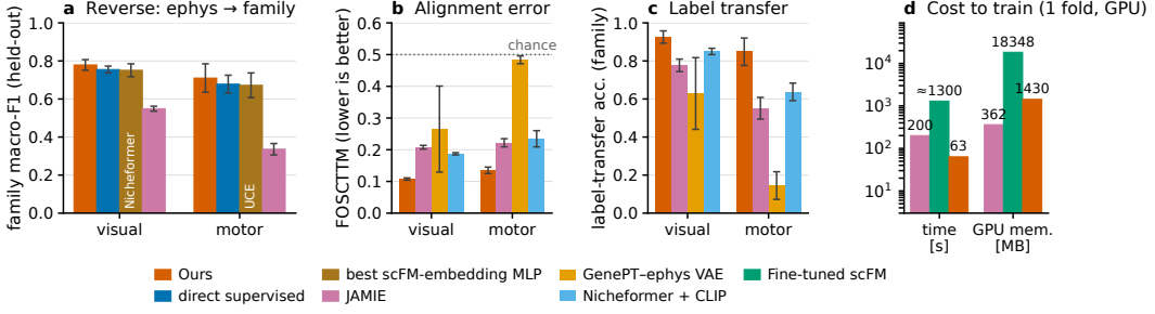
Figure 2: Shared space. (a) Reverse readout of transcriptomic family from electrophysiology (macro-F1). (b) Held-out FOSCTTM (lower is better; 0.5 is chance) and (c) family label-transfer accuracy for the methods that expose a joint space, JAMIE re-run on our folds. (d) Training time and peak GPU memory comparisons for one fold, cost-efficiency (Appendix C)
