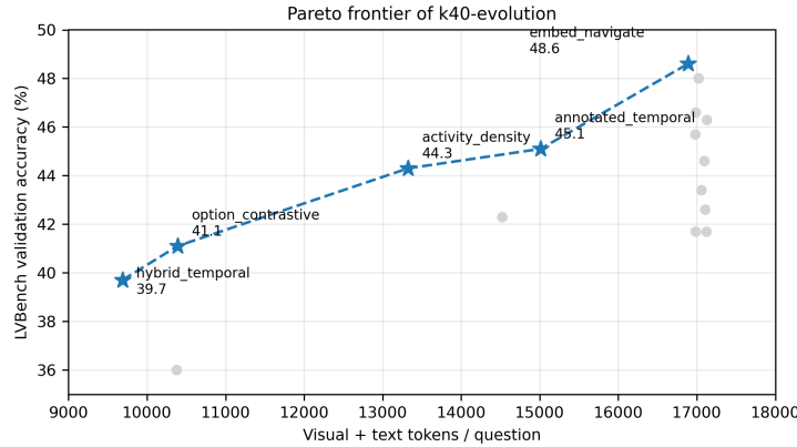
Figure 3: Development accuracy versus estimated visual-plus-text input tokens per question for the K = 40 search. The Pareto view separates maximum accuracy from lower-cost candidate programs; gray points are dominated candidates.
