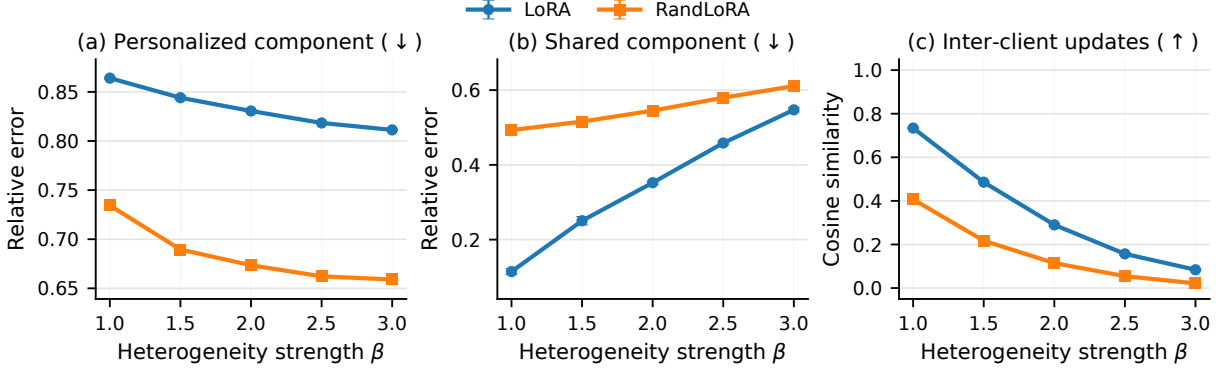
Figure 2: Controlled comparison of LoRA and RandLoRA under increasing client heterogeneity. Panels report (a) personalization error, (b) aggregation error, and (c) mean cross-client update similarity.
