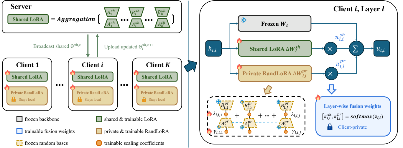
Figure 3: Overview of the FedLAFP framework. (a) The server broadcasts the shared LoRA parameters, and clients upload only their locally updated shared parameters for sample-weighted aggregation, while the private RandLoRA parameters remain local. (b) Within target layer \ell of client i , the output of the frozen linear transformation is augmented by the weighted outputs of the shared LoRA and private RandLoRA branches, using \pi_{\ell,i}^{\text{sh}} and \pi_{\ell,i}^{\text{pr}} , respectively. These client- and layer-specific fusion weights are derived from private logits and are never communicated.
