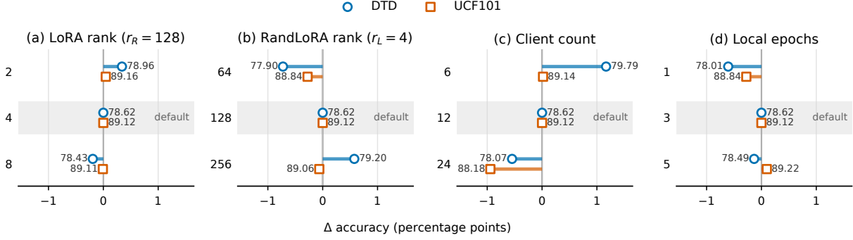
Figure 5: Hyperparameter sensitivity on DTD and UCF101. Each panel varies one hyperparameter while holding the remaining settings fixed. The horizontal axis shows the accuracy change in percentage points relative to the default configuration ( r_L, r_R, K, E ) = (4, 128, 12, 3); marker labels show absolute accuracy (%). The shaded row denotes the default value.
