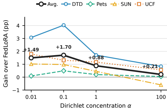
Figure 6: Accuracy gain of FedLAFP over FedLoRA under different Dirichlet concentration parameters. Positive values indicate an improvement over FedLoRA under the same client partition. The black curve shows the mean gain across the four datasets; larger \alpha corresponds to less heterogeneous client data.
