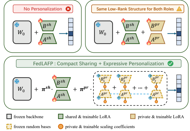
Figure 1: Comparison of global-only adaptation, symmetric shared-private LoRA, and the proposed role-aware FedLAFP.
