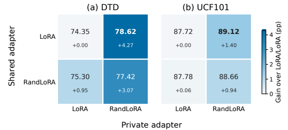
Figure 4: Role-assignment matrices on DTD and UCF101. Rows specify the shared adapter and columns specify the private adapter. Each cell reports accuracy (%); the smaller annotation and cell color encode the gain over LoRA/LoRA. Bold values denote the best assignment per dataset.
